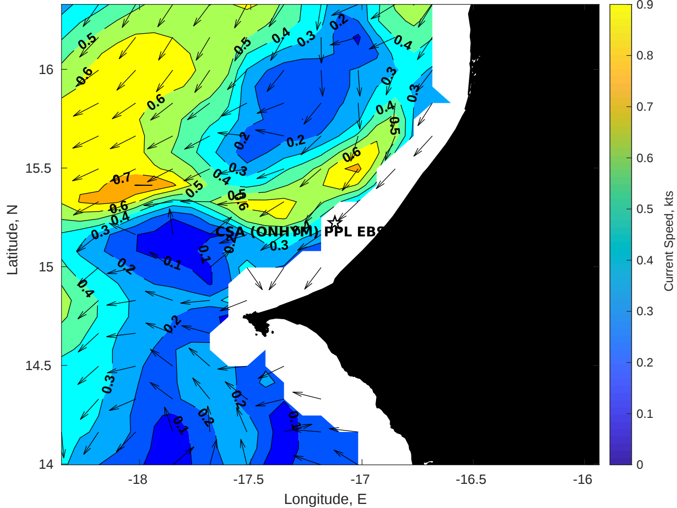
Surface Currents for CSA (ONHYM) PPL EBS - Senegal at 14-Jan-2026 00:00:00
