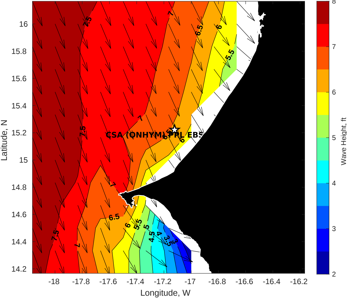
GFS Wave Height (ft) for CSA (ONHYM) PPL EBS - Senegal at 15-Jan-2026 09:00:00
