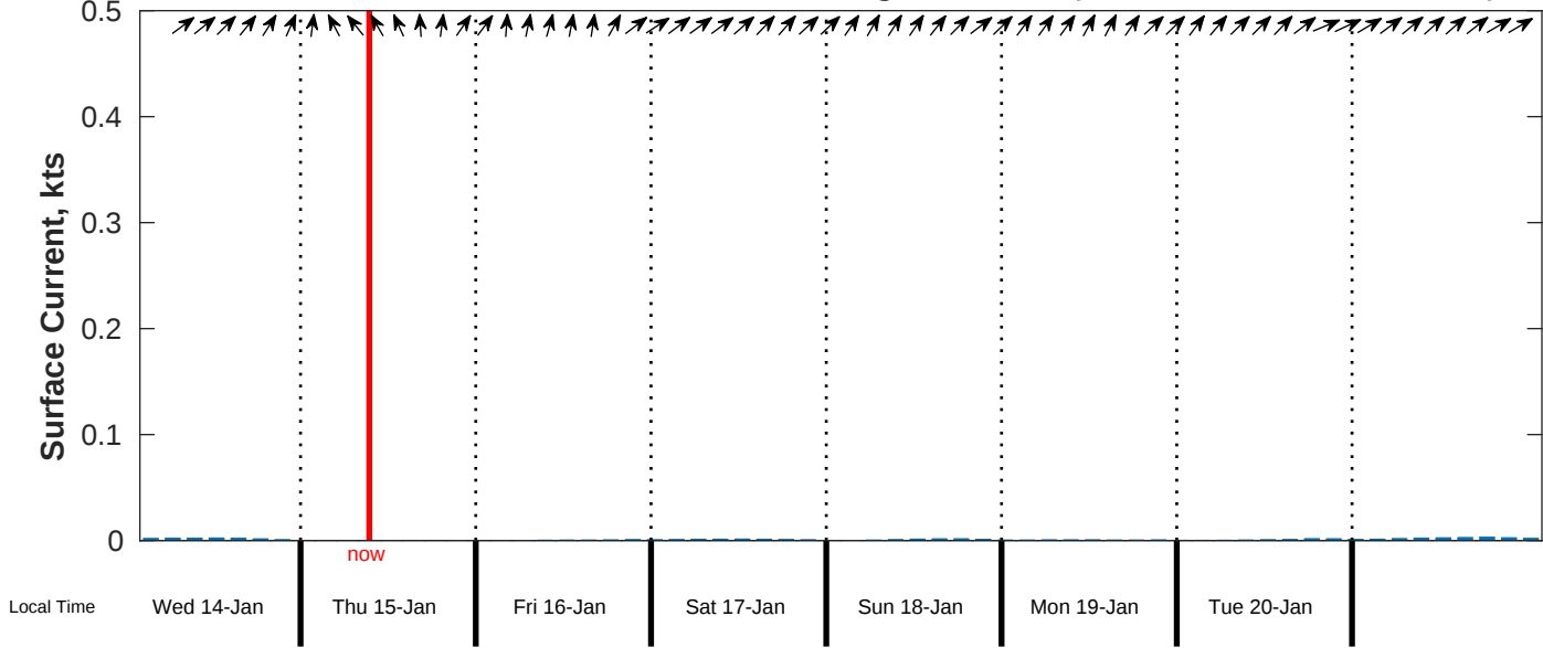
Surface Current Forecast for CSA (ONHYM) PPL EBS - Senegal from 14-Jan-2026 00:00:00 to 22-Jan-2026 00:00:00
