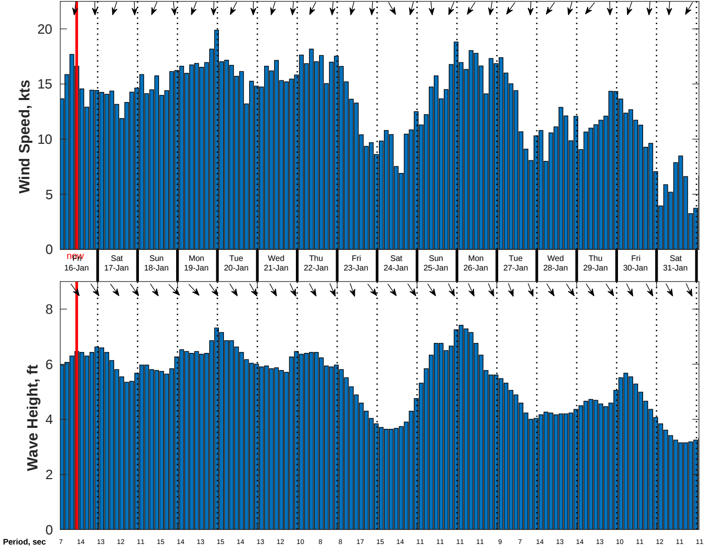
Wind & Wave Forecast for CSA (ONHYM) PPL EBS - Senegal from 15-Jan-2026 01:00:00 to 31-Jan-2026 01:00:00
