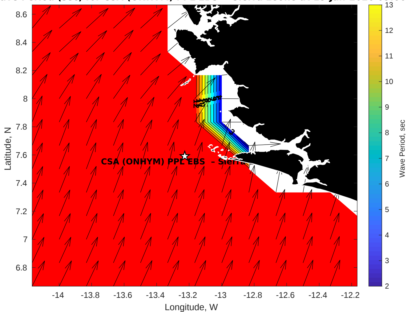
GFS Wave Period (sec) for CSA (ONHYM) PPL EBS - Sierra Leone at 15-Jan-2026 09:00:00
