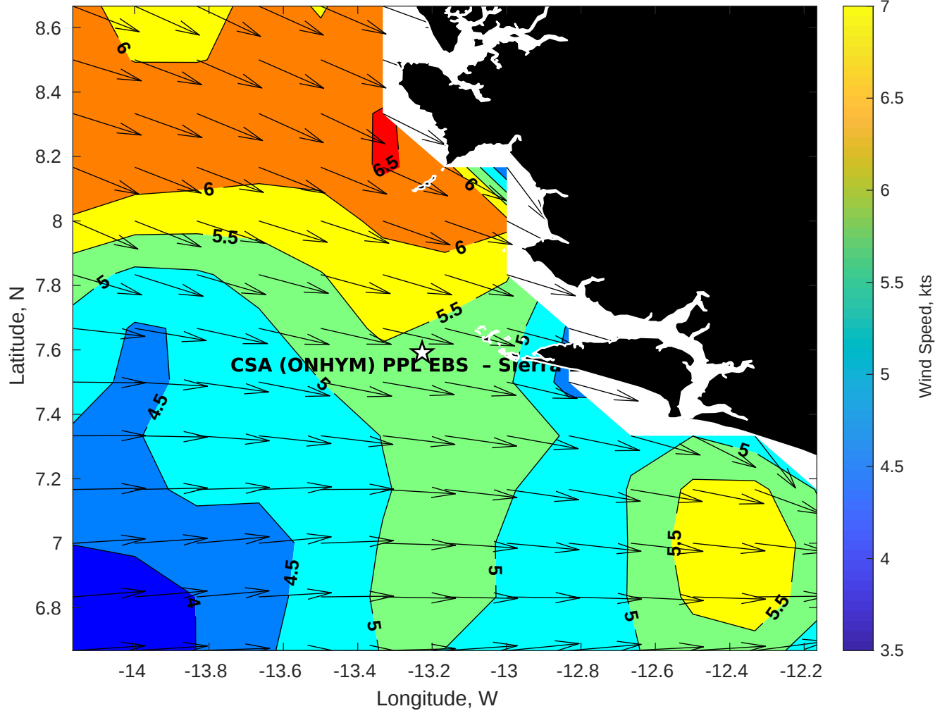
GFS Winds (kts) for CSA (ONHYM) PPL EBS - Sierra Leone at 15-Jan-2026 09:00:00
