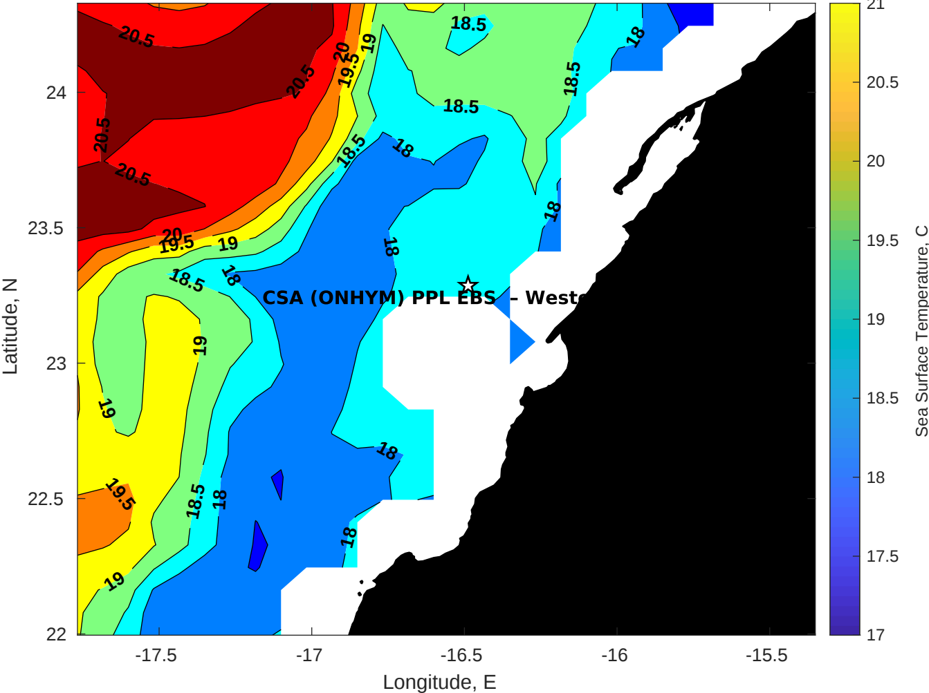
SST for CSA (ONHYM) PPL EBS - Western Sahara at 14-Jan-2026 00:00:00
