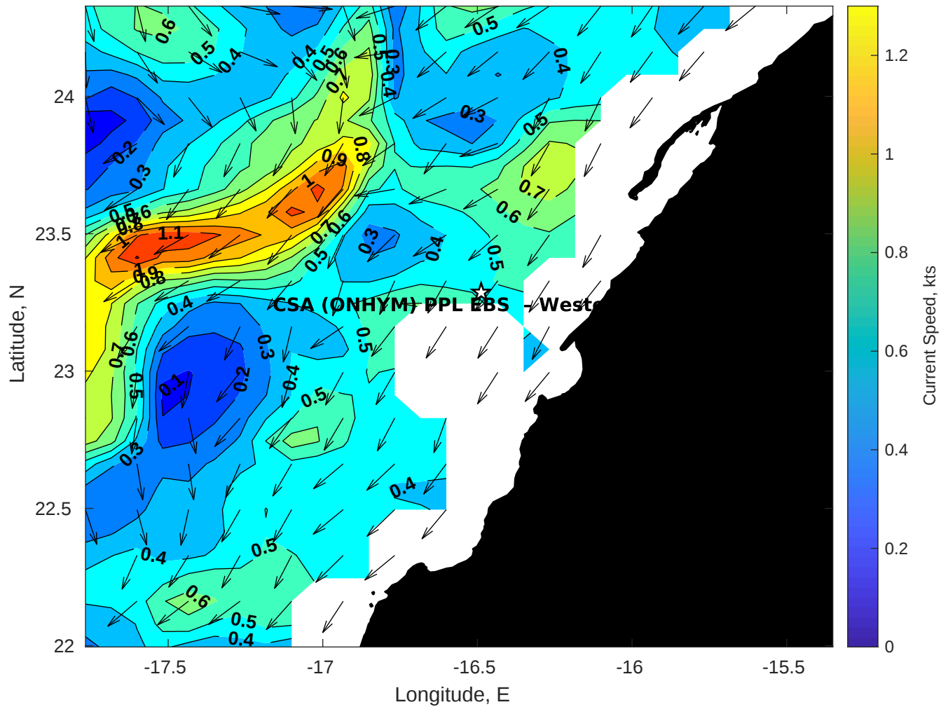
Surface Currents for CSA (ONHYM) PPL EBS - Western Sahara at 14-Jan-2026 00:00:00
