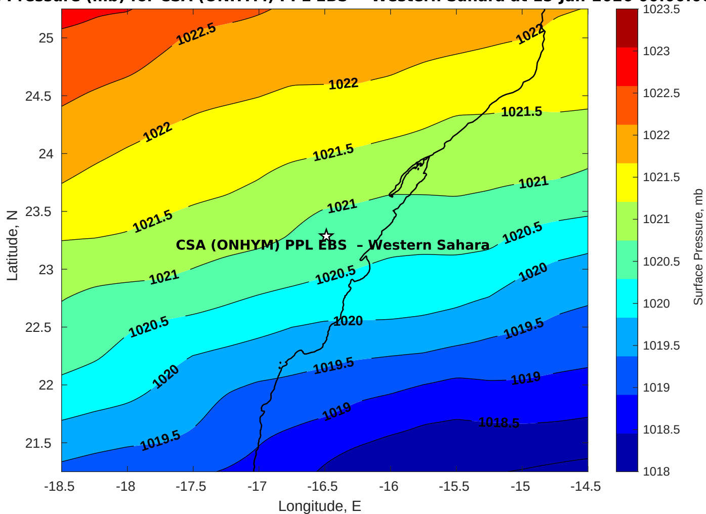
Surface Pressure (mb) for CSA (ONHYM) PPL EBS - Western Sahara at 15-Jan-2026 00:00:00
