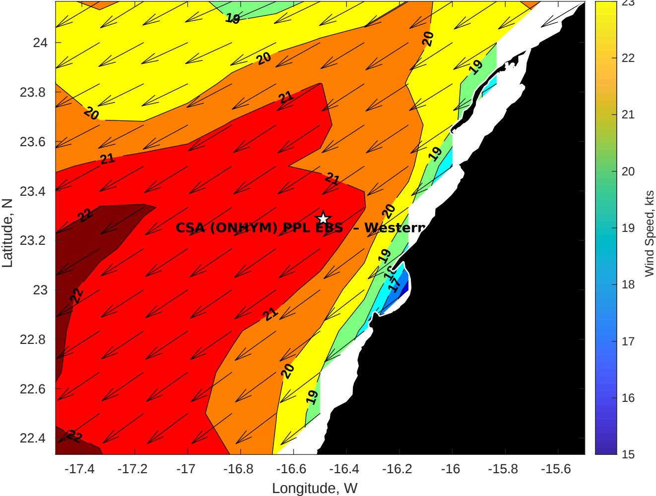
GFS Winds (kts) for CSA (ONHYM) PPL EBS - Western Sahara at 15-Jan-2026 09:00:00
