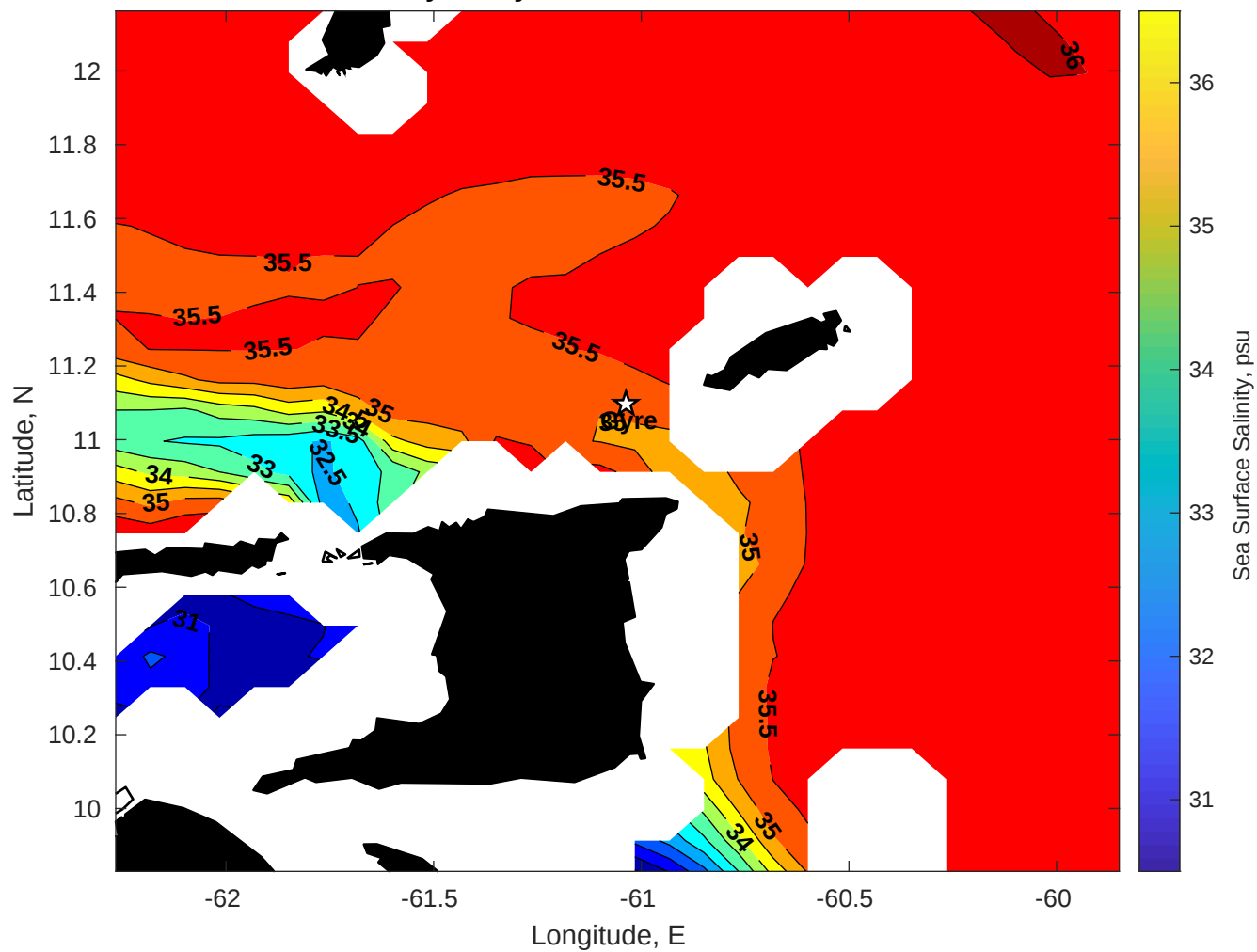
Surface Salinity for Gyre at 14-Jan-2026 00:00:00
