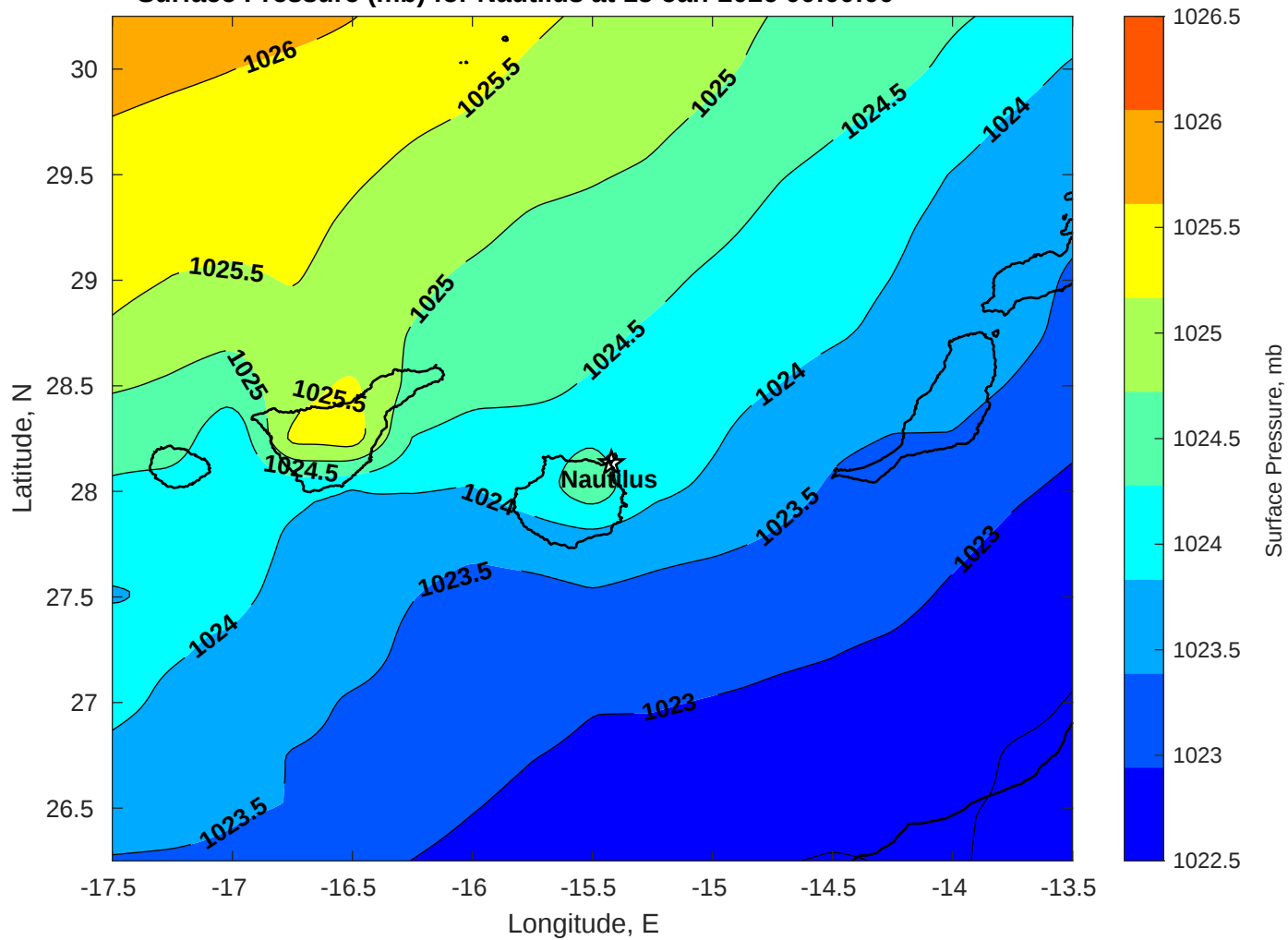
Surface Pressure (mb) for Nautilus at 15-Jan-2026 00:00:00
