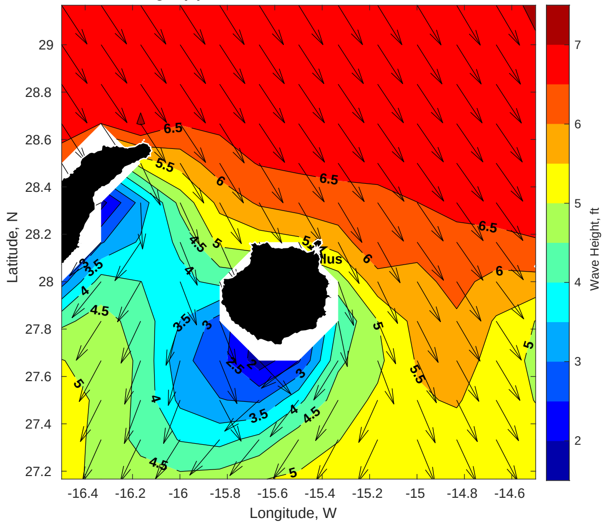
GFS Wave Height (ft) for Nautilus at 15-Jan-2026 09:00:00
