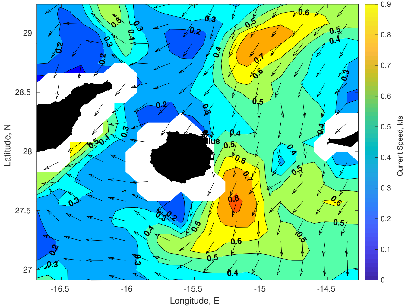
Surface Currents for Nautilus at 14-Jan-2026 00:00:00
