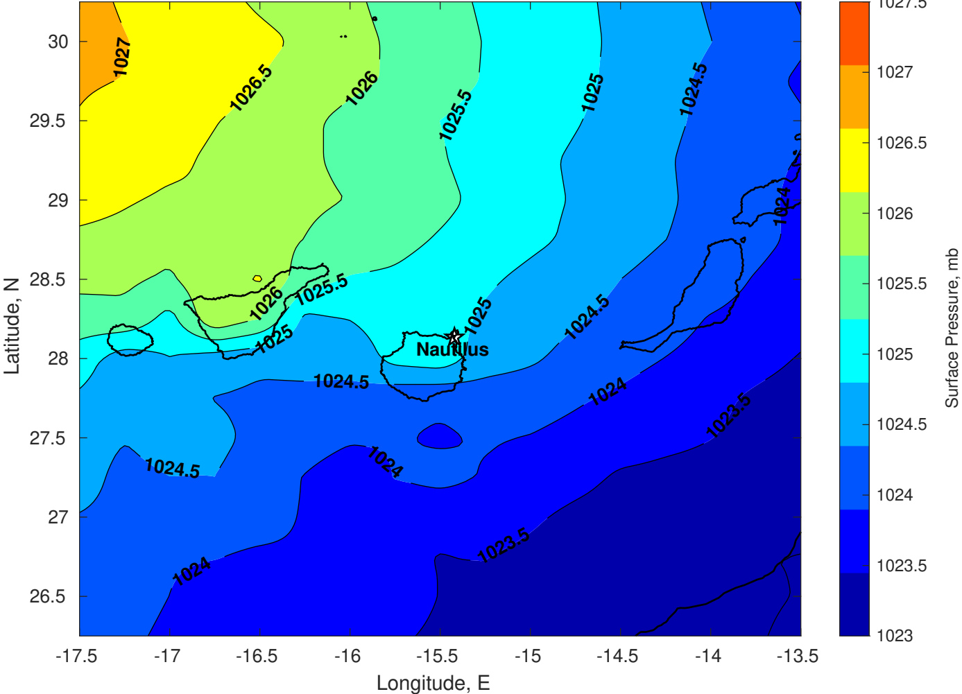
Surface Pressure (mb) for Nautilus at 17-Jan-2026 00:00:00
