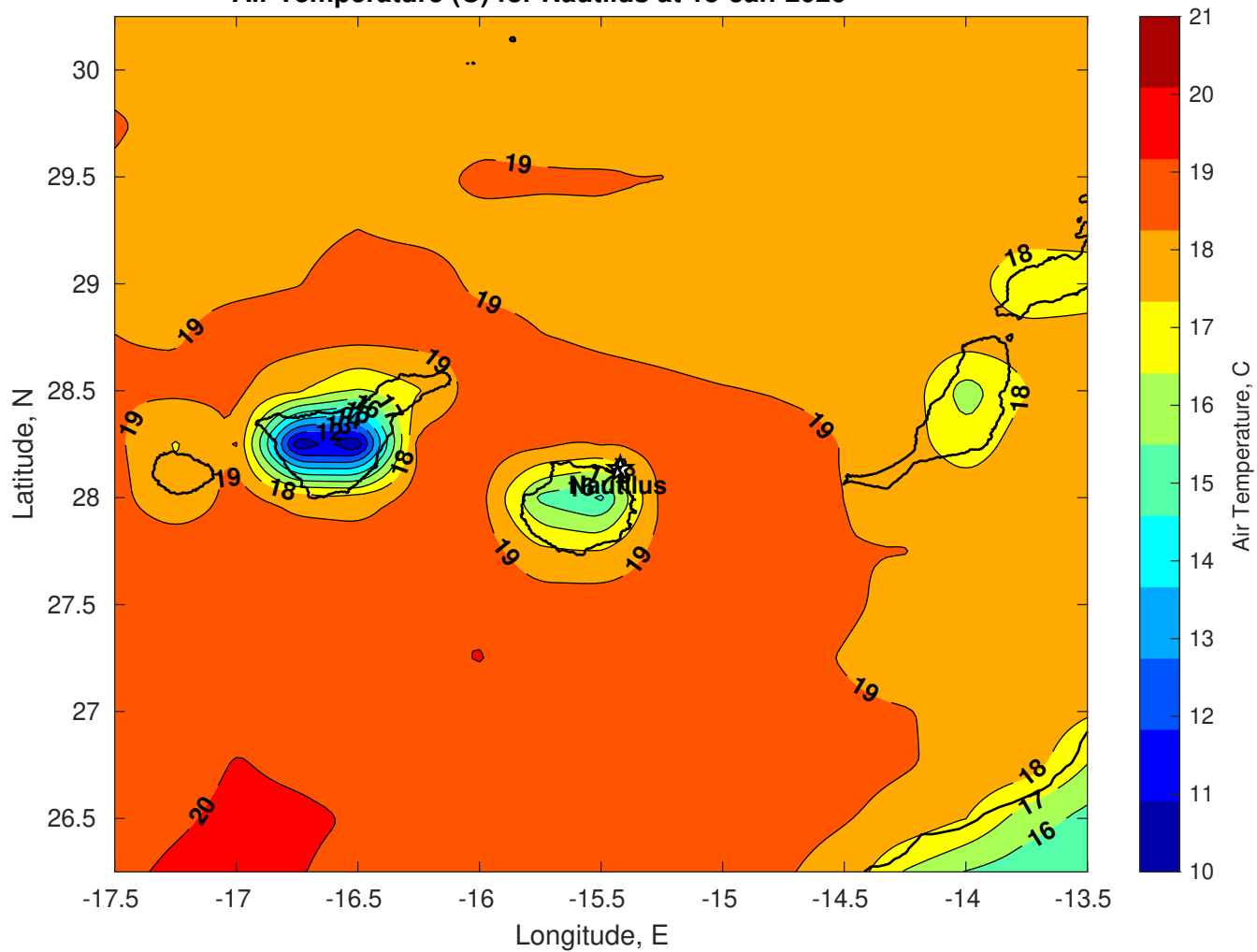
Air Temperature (C) for Nautilus at 15-Jan-2026
