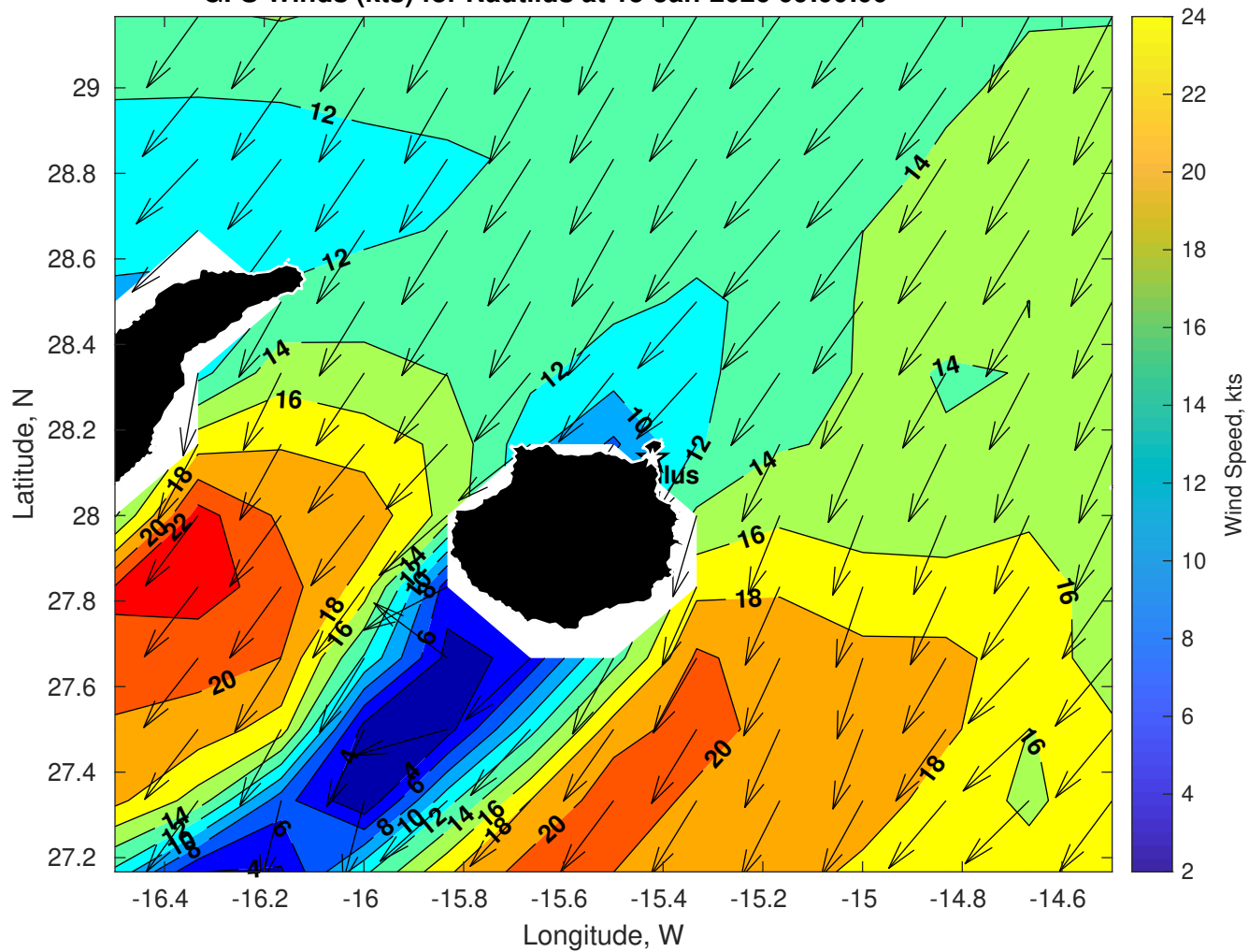
GFS Winds (kts) for Nautilus at 15-Jan-2026 09:00:00
