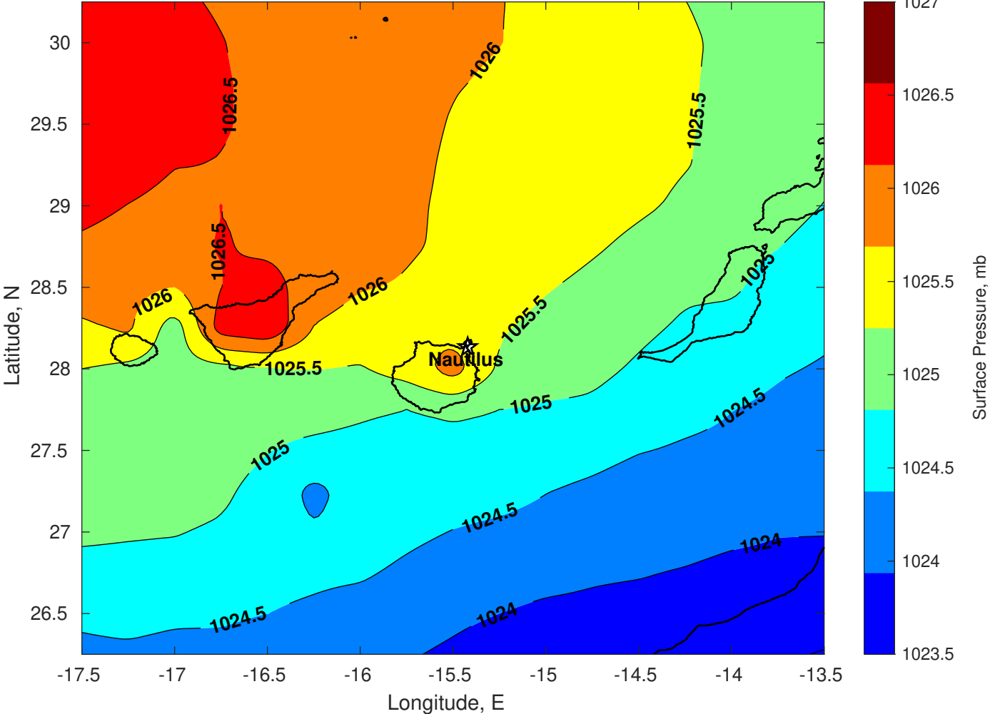
Surface Pressure (mb) for Nautilus at 16-Jan-2026 00:00:00
