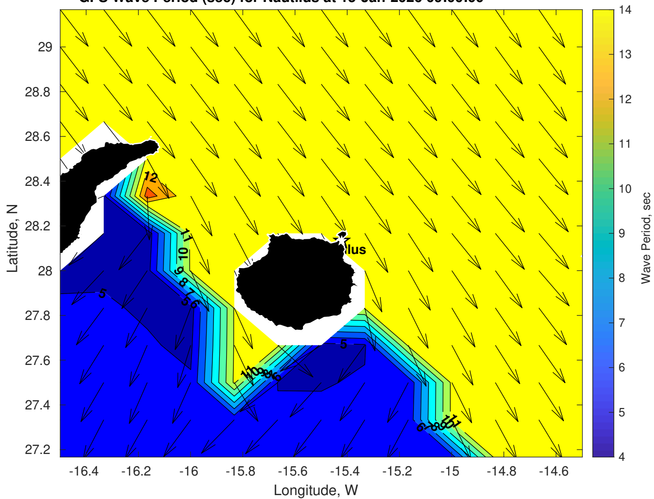
GFS Wave Period (sec) for Nautilus at 15-Jan-2026 09:00:00
