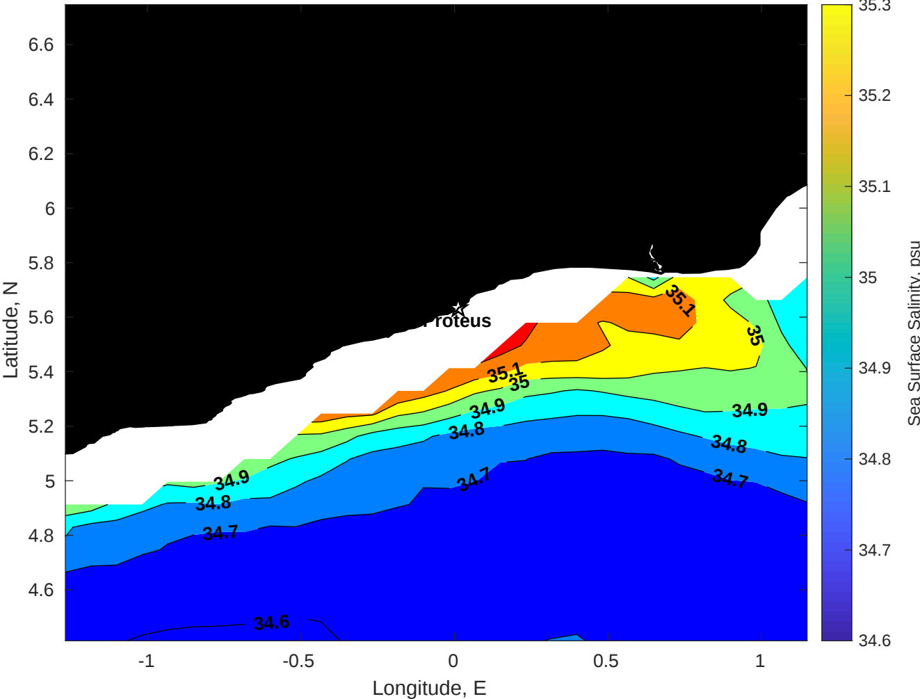
Surface Salinity for Proteus at 14-Jan-2026 00:00:00
