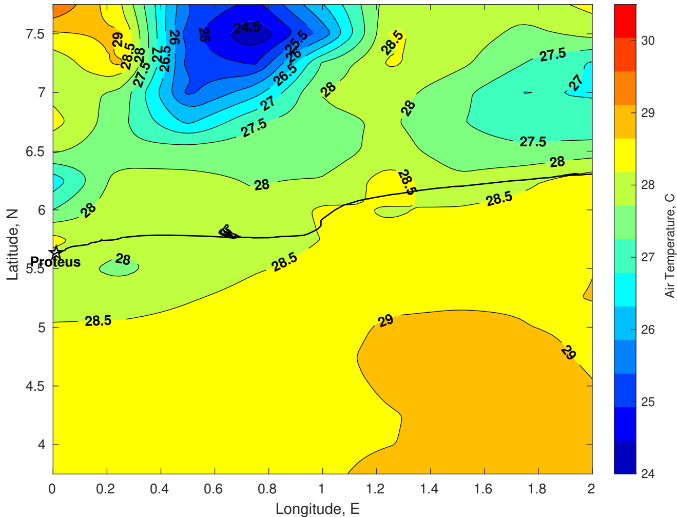
Air Temperature (C) for Proteus at 15-Jan-2026
