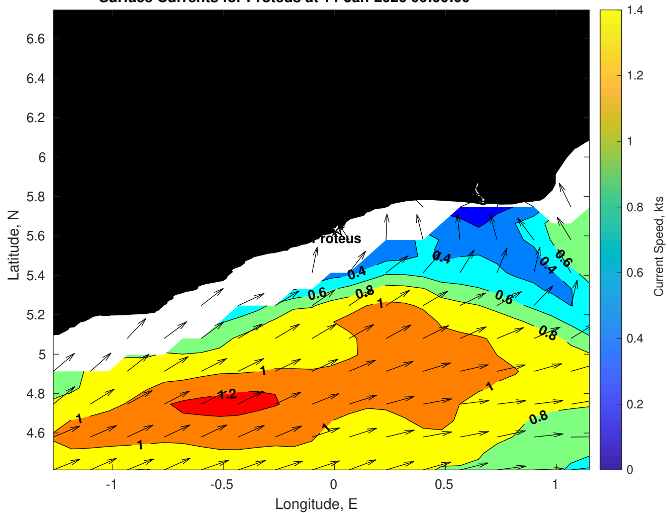
Surface Currents for Proteus at 14-Jan-2026 00:00:00
