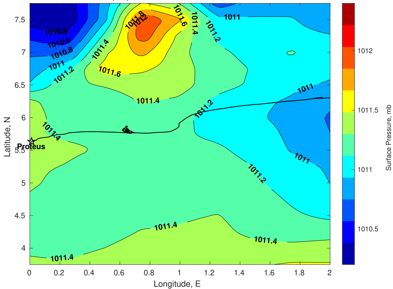
Surface Pressure (mb) for Proteus at 16-Jan-2026 00:00:00
