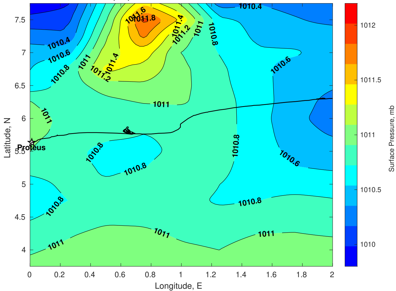
Surface Pressure (mb) for Proteus at 15-Jan-2026 00:00:00
