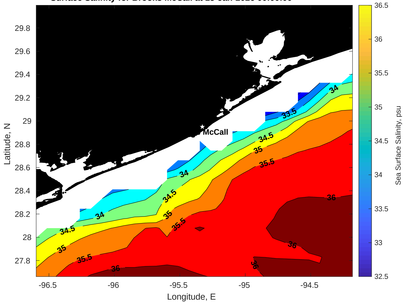
Surface Salinity for Brooks McCall at 15-Jan-2026 00:00:00
