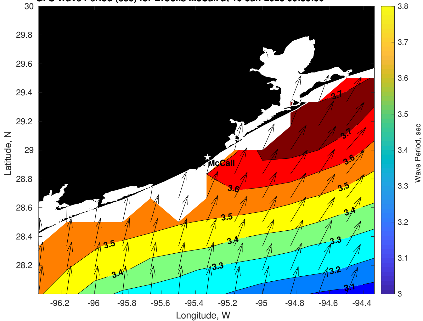
GFS Wave Period (sec) for Brooks McCall at 16-Jan-2026 09:00:00
