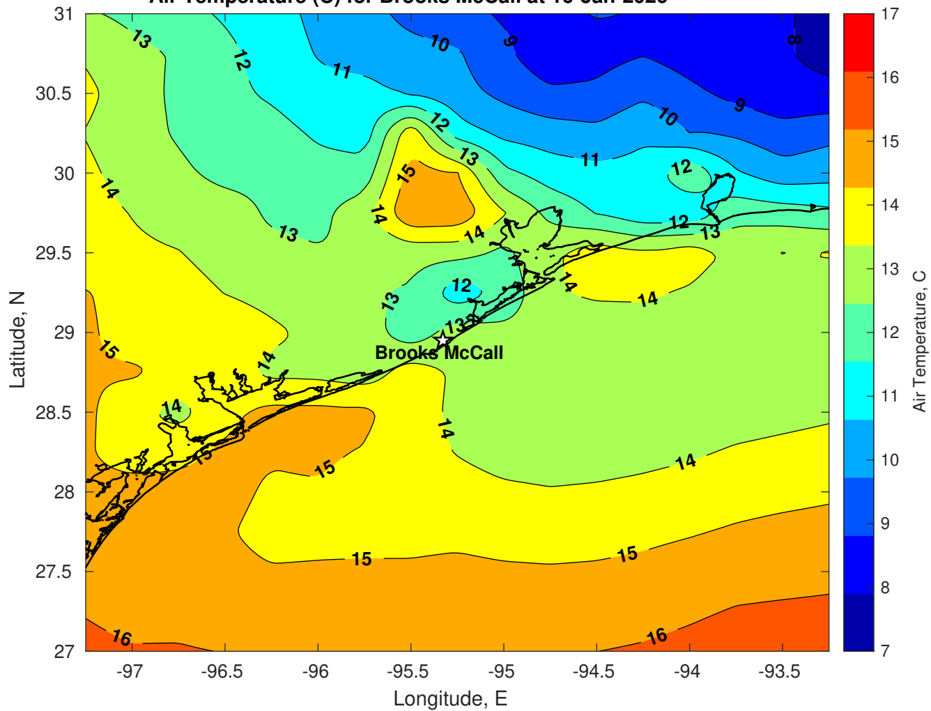
Air Temperature (C) for Brooks McCall at 16-Jan-2026
