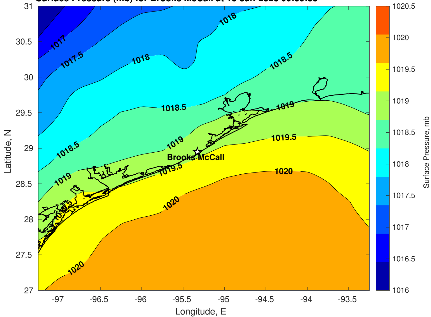
Surface Pressure (mb) for Brooks McCall at 16-Jan-2026 00:00:00
