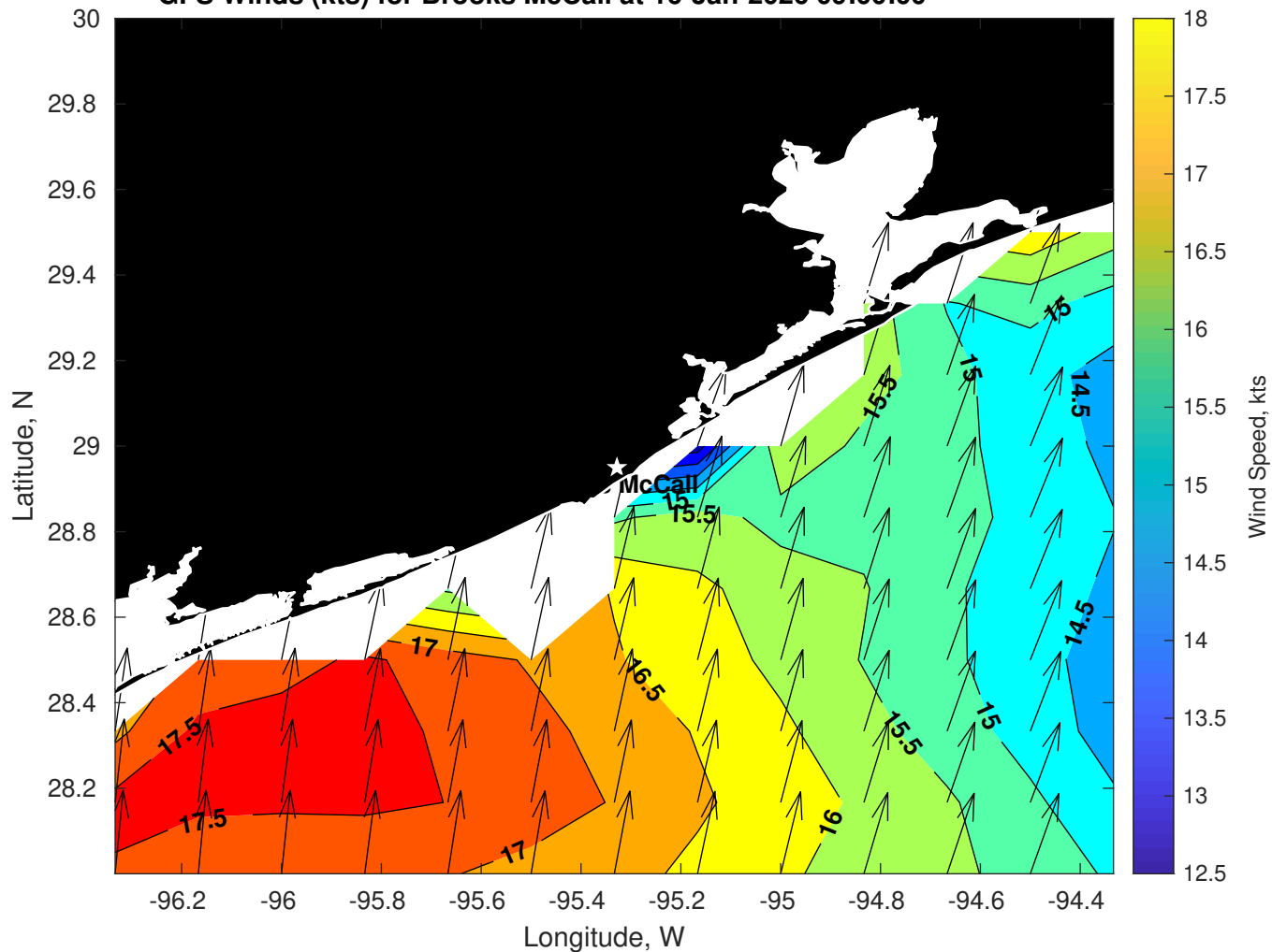
GFS Winds (kts) for Brooks McCall at 16-Jan-2026 09:00:00
