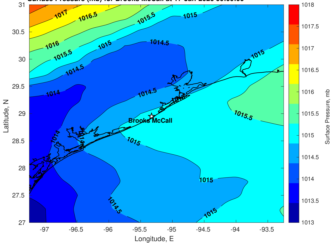
Surface Pressure (mb) for Brooks McCall at 17-Jan-2026 00:00:00
