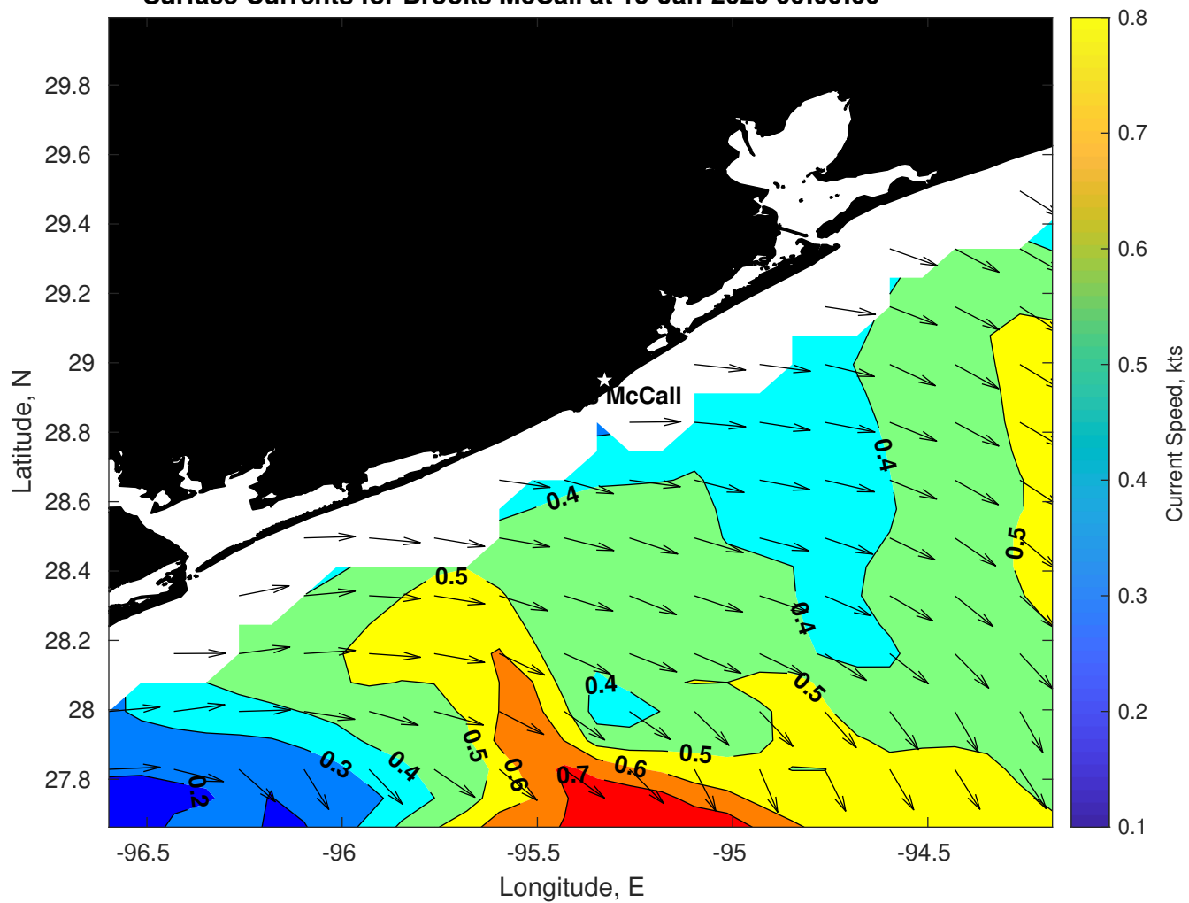
Surface Currents for Brooks McCall at 15-Jan-2026 00:00:00
