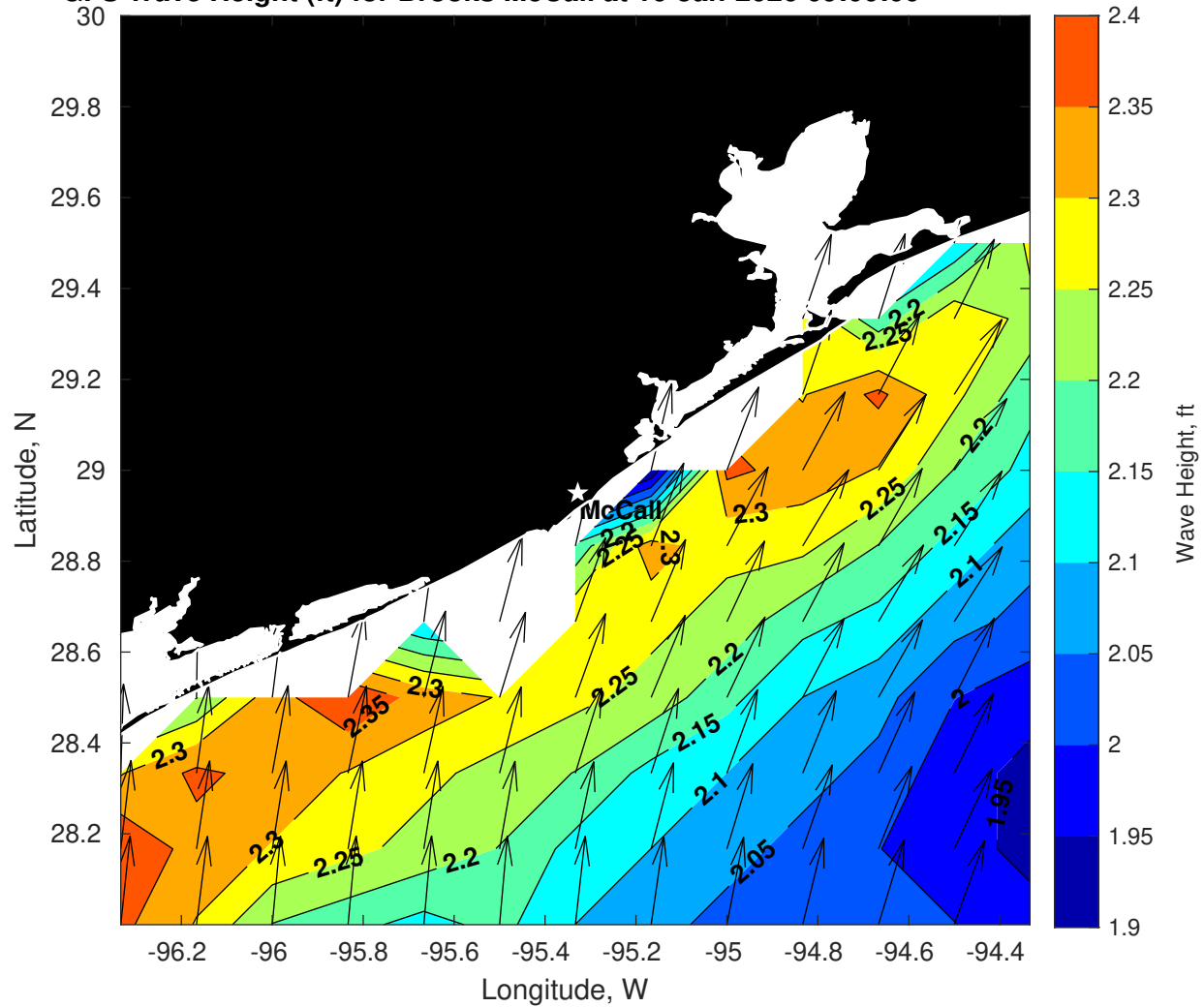
GFS Wave Height (ft) for Brooks McCall at 16-Jan-2026 09:00:00
