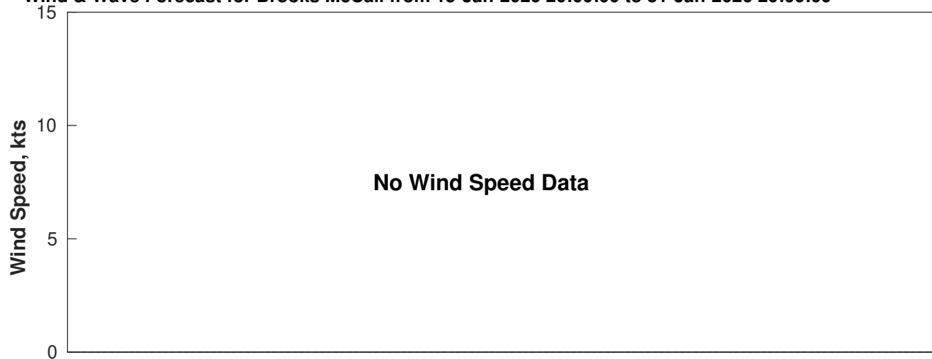
Wind & Wave Forecast for Brooks McCall from 15-Jan-2026 20:00:00 to 31-Jan-2026 20:00:00
