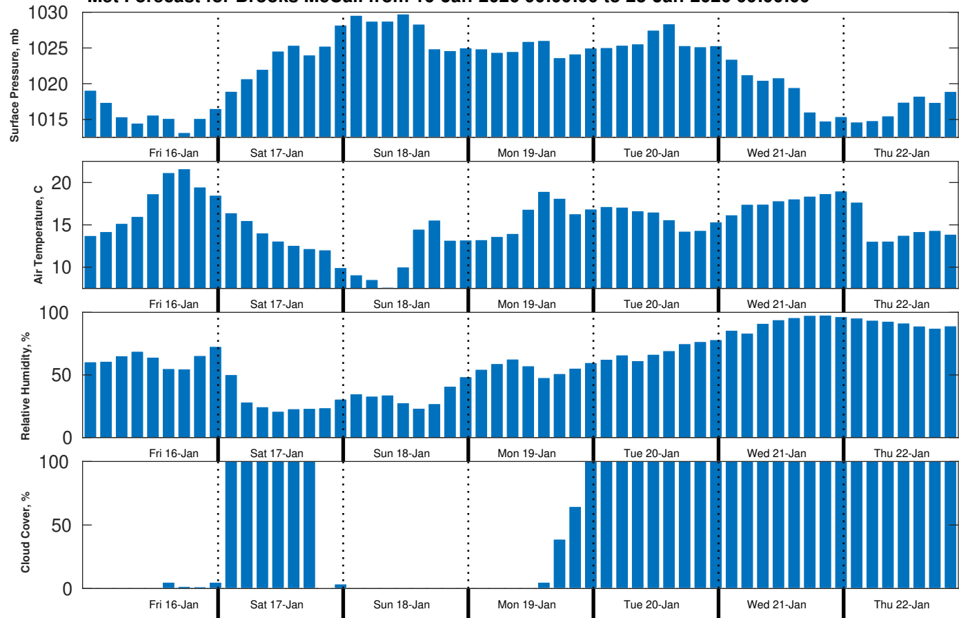
Met Forecast for Brooks McCall from 16-Jan-2026 00:00:00 to 23-Jan-2026 00:00:00
