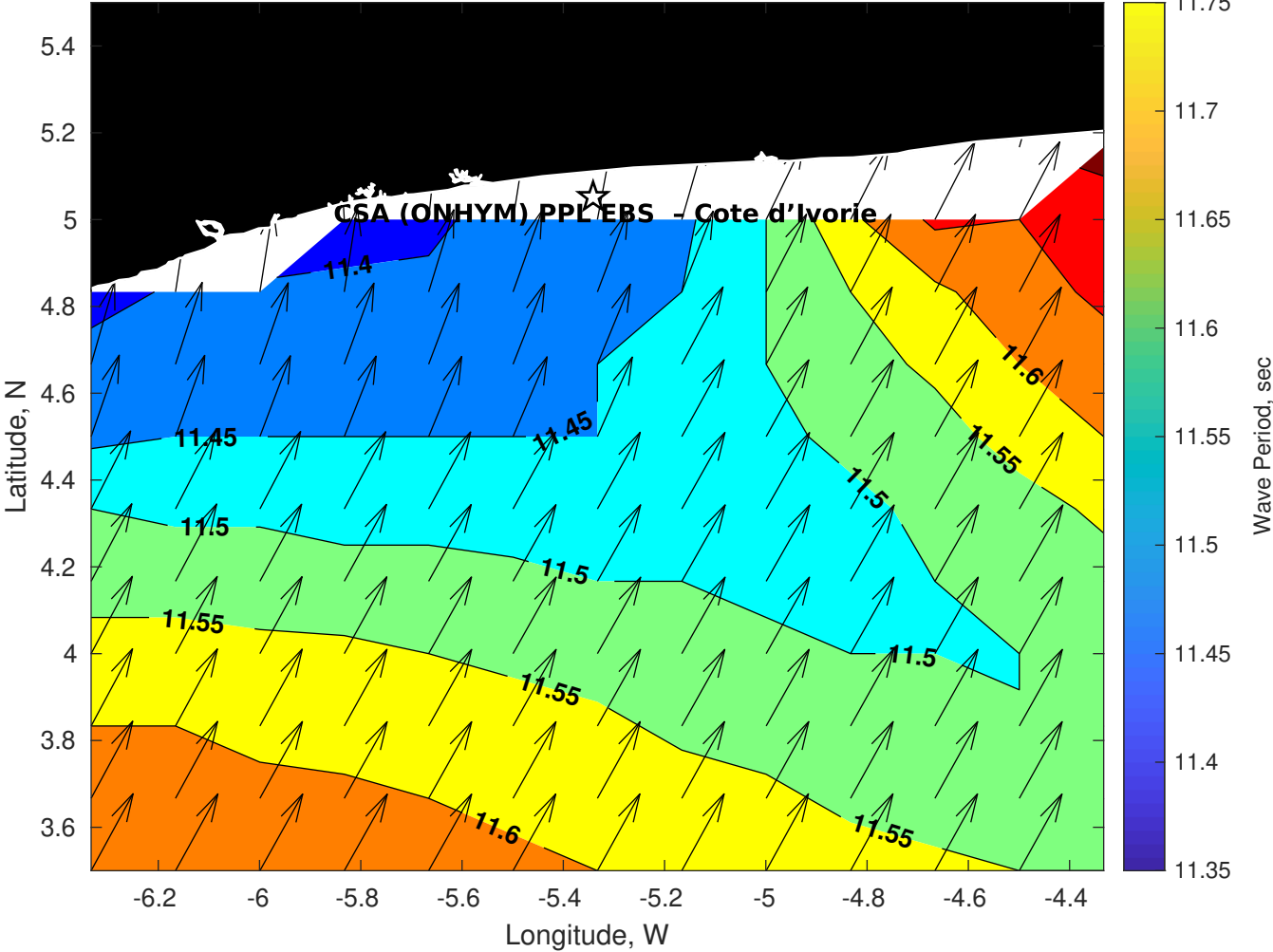
GFS Wave Period (sec) for CSA (ONHYM) PPL EBS - Cote d'Ivoire at 16-Jan-2026 09:00:00
