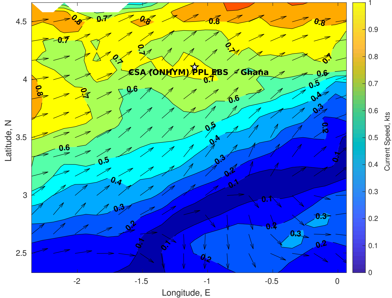
Surface Currents for CSA (ONHYM) PPL EBS - Ghana at 15-Jan-2026 00:00:00
