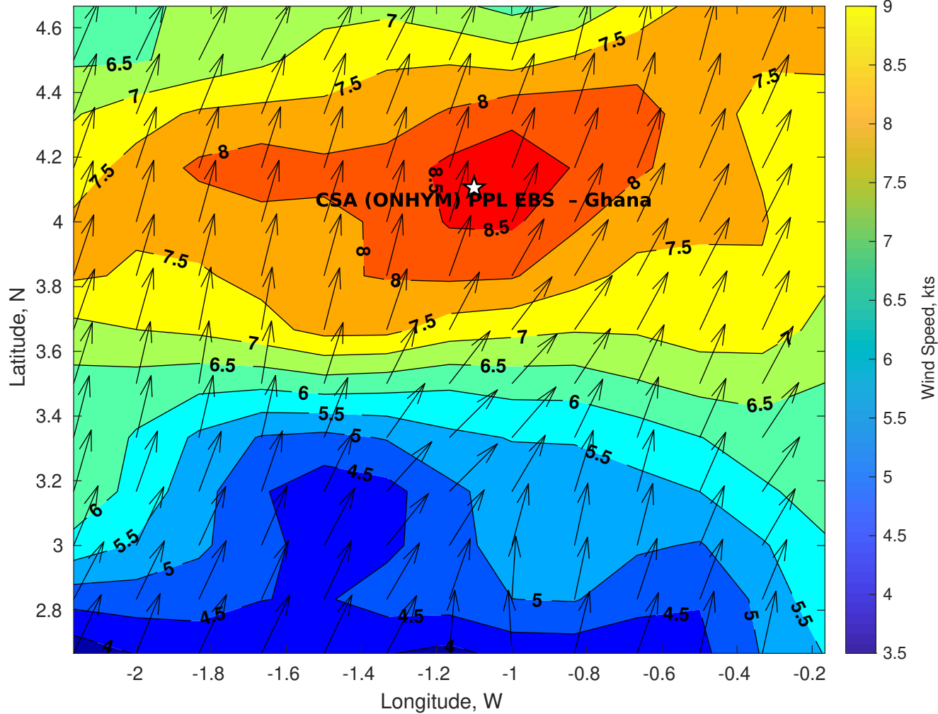
GFS Winds (kts) for CSA (ONHYM) PPL EBS - Ghana at 16-Jan-2026 09:00:00
