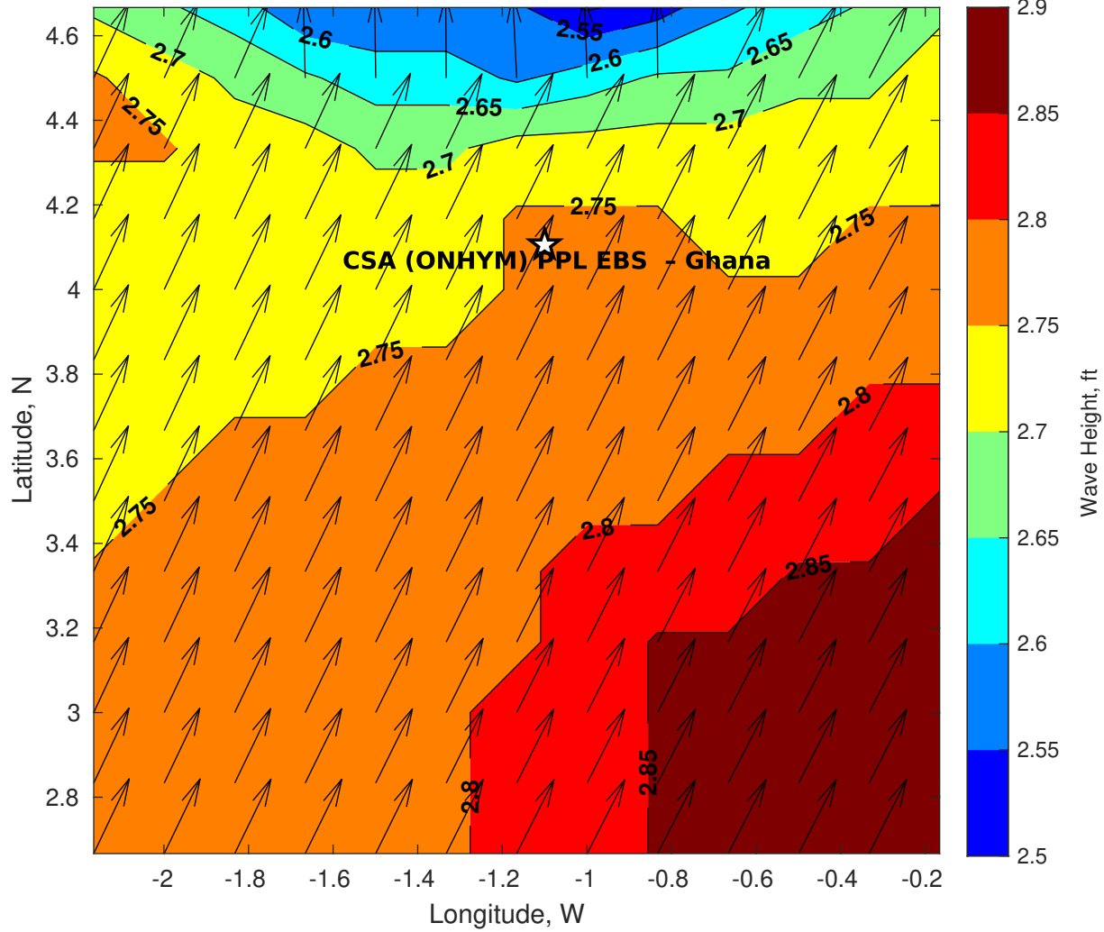
GFS Wave Height (ft) for CSA (ONHYM) PPL EBS - Ghana at 16-Jan-2026 09:00:00
