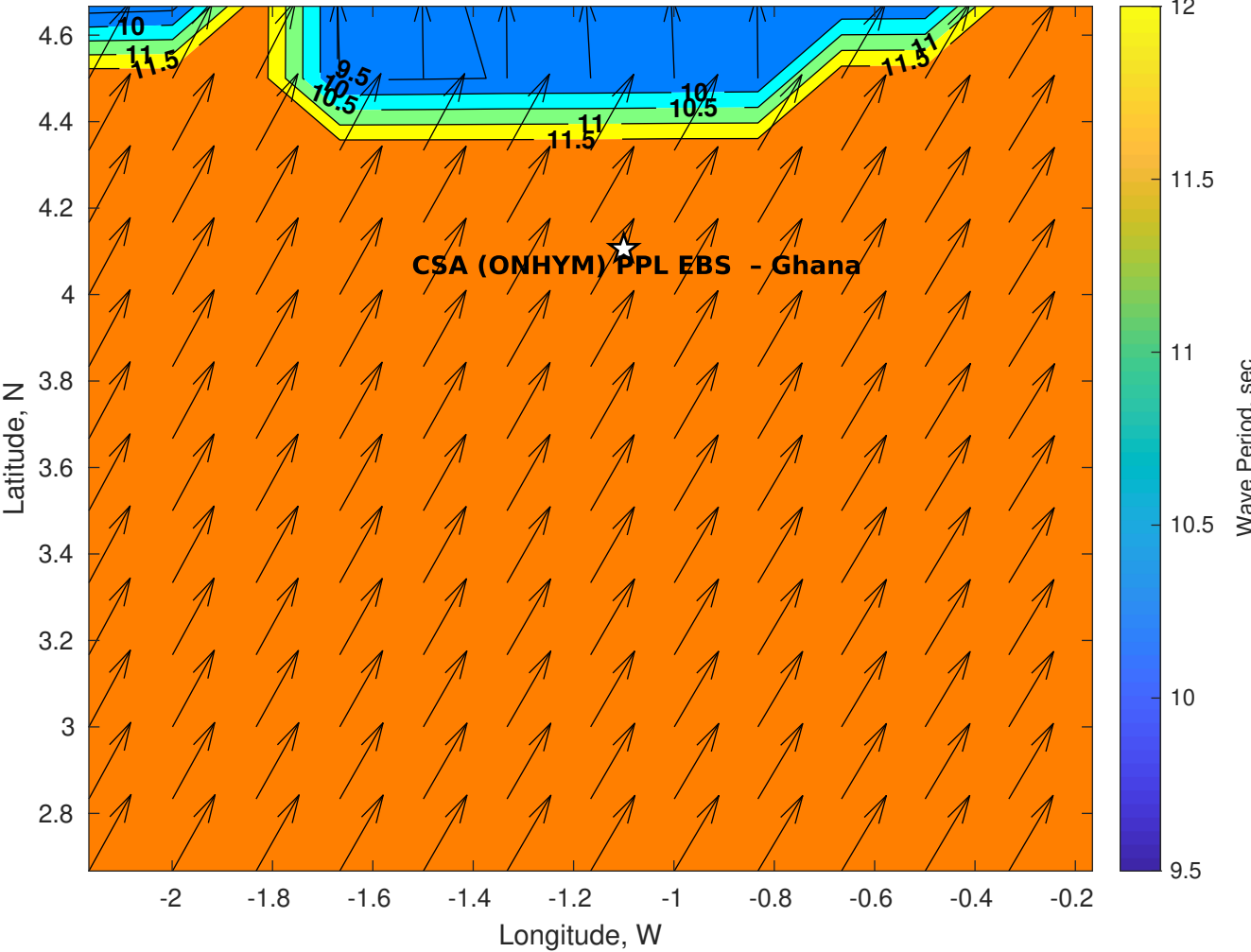
GFS Wave Period (sec) for CSA (ONHYM) PPL EBS - Ghana at 16-Jan-2026 09:00:00
