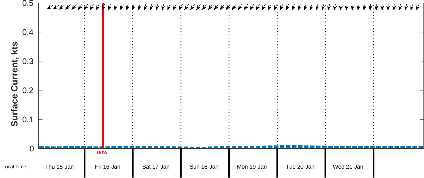
Surface Current Forecast for CSA (ONHYM) PPL EBS - Ghana from 15-Jan-2026 00:00:00 to 23-Jan-2026 00:00:00
