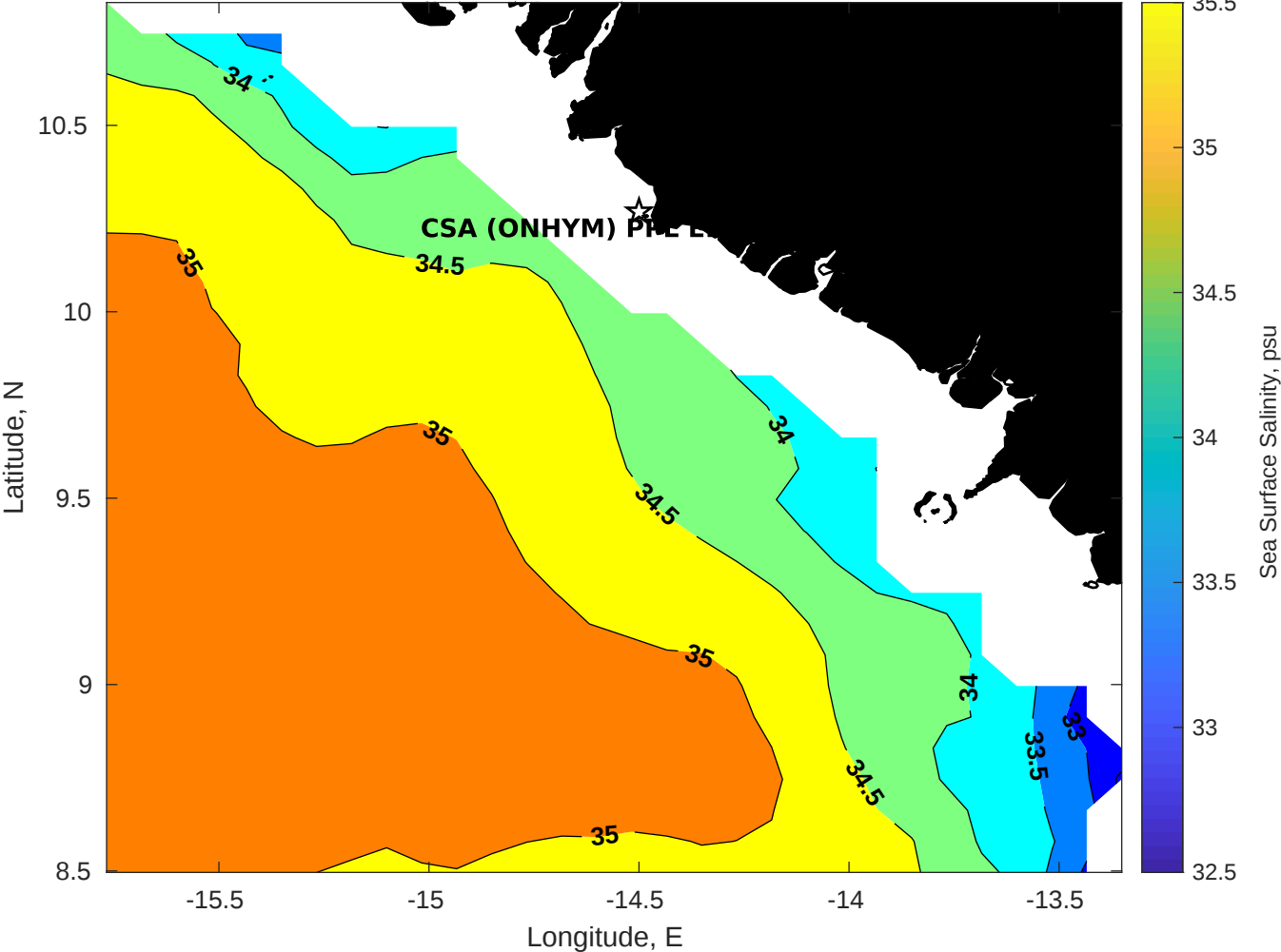
Surface Salinity for CSA (ONHYM) PPL EBS - Guinea at 15-Jan-2026 00:00:00
