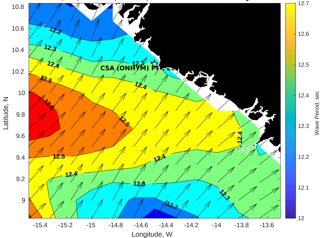
GFS Wave Period (sec) for CSA (ONHYM) PPL EBS - Guinea at 16-Jan-2026 09:00:00
