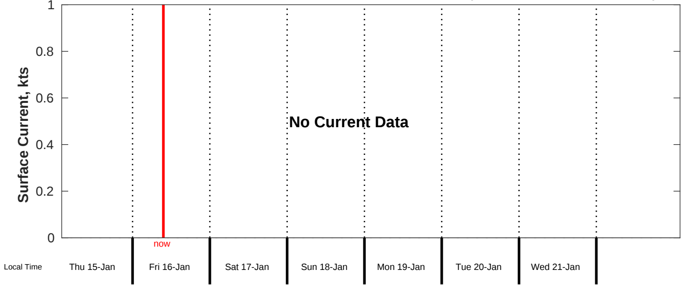
Surface Current Forecast for CSA (ONHYM) PPL EBS - Guinea from 15-Jan-2026 00:00:00 to 23-Jan-2026 00:00:00
