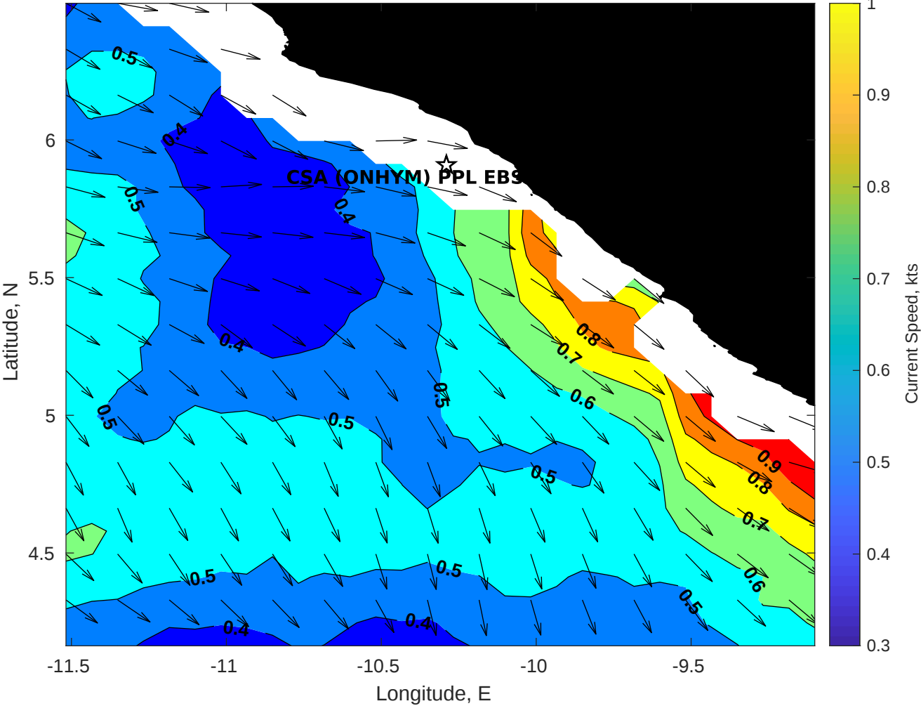
Surface Currents for CSA (ONHYM) PPL EBS - Liberia at 15-Jan-2026 00:00:00
