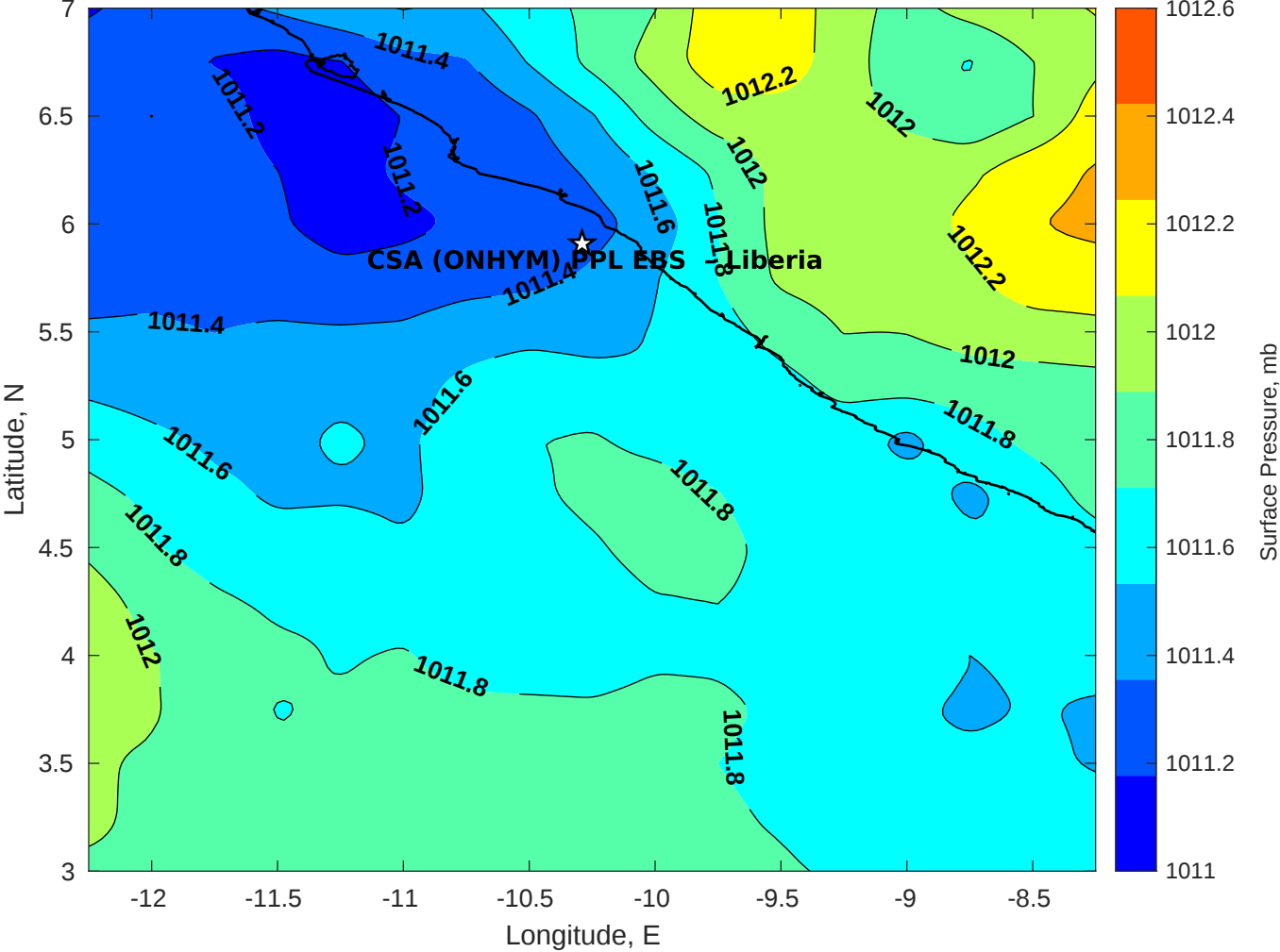
Surface Pressure (mb) for CSA (ONHYM) PPL EBS - Liberia at 16-Jan-2026 00:00:00
