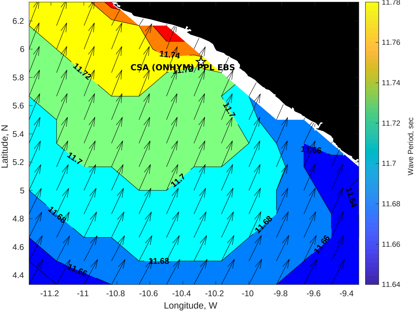
GFS Wave Period (sec) for CSA (ONHYM) PPL EBS - Liberia at 16-Jan-2026 09:00:00
