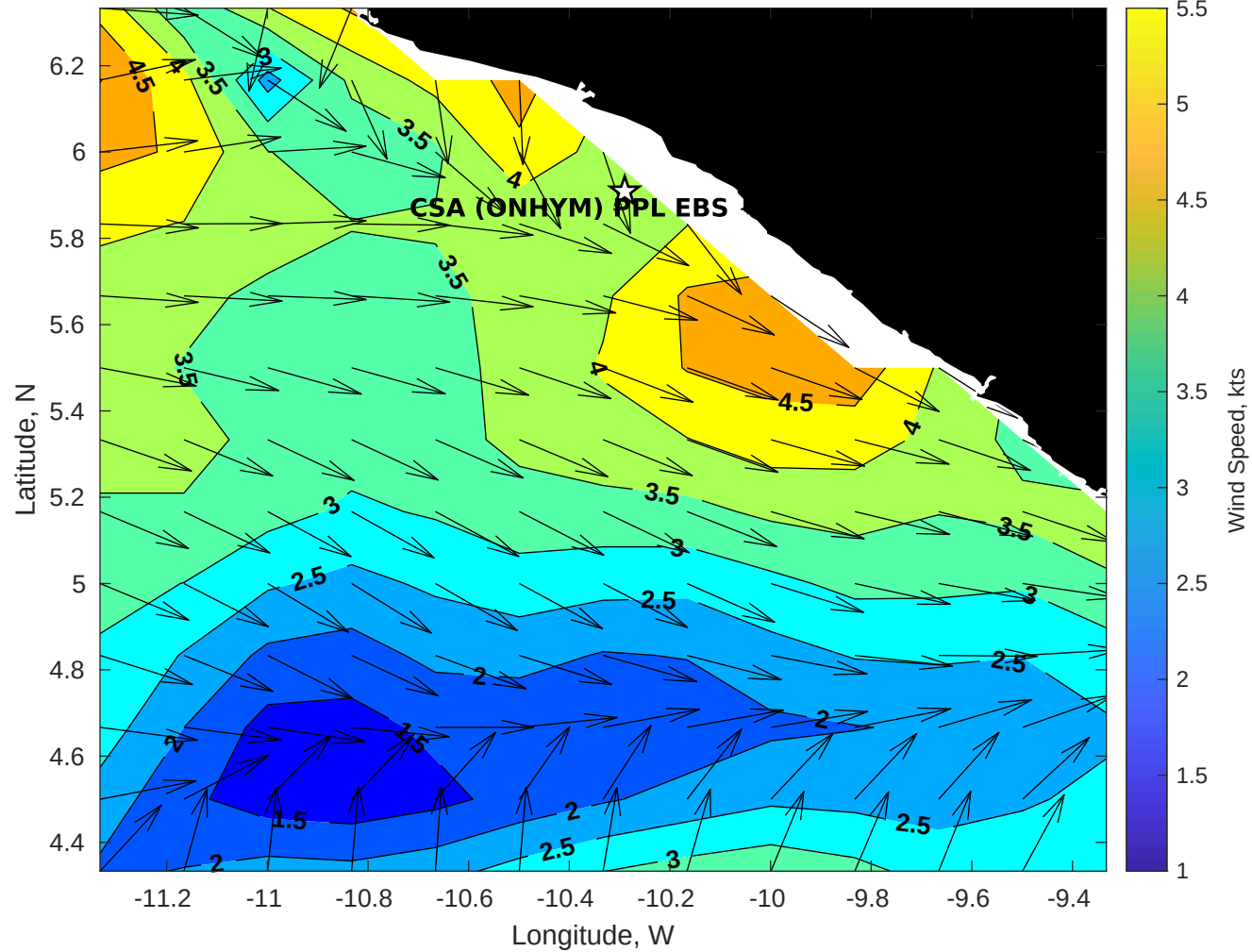
GFS Winds (kts) for CSA (ONHYM) PPL EBS - Liberia at 16-Jan-2026 09:00:00
