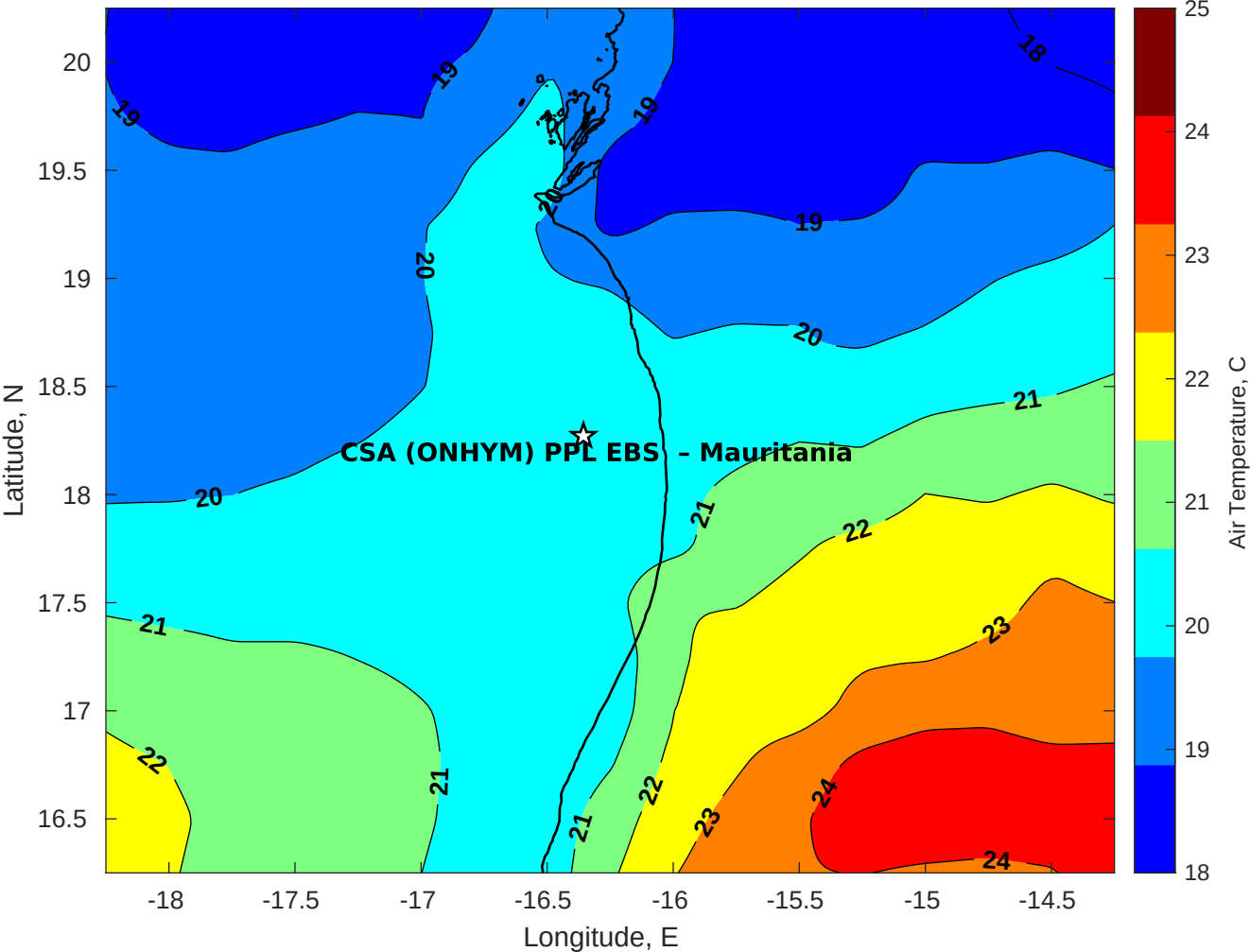
Air Temperature (C) for CSA (ONHYM) PPL EBS - Mauritania at 16-Jan-2026
