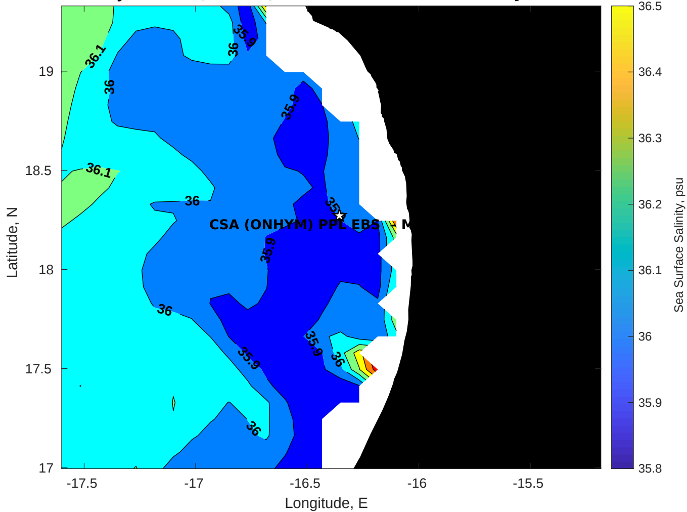
Surface Salinity for CSA (ONHYM) PPL EBS - Mauritania at 15-Jan-2026 00:00:00
