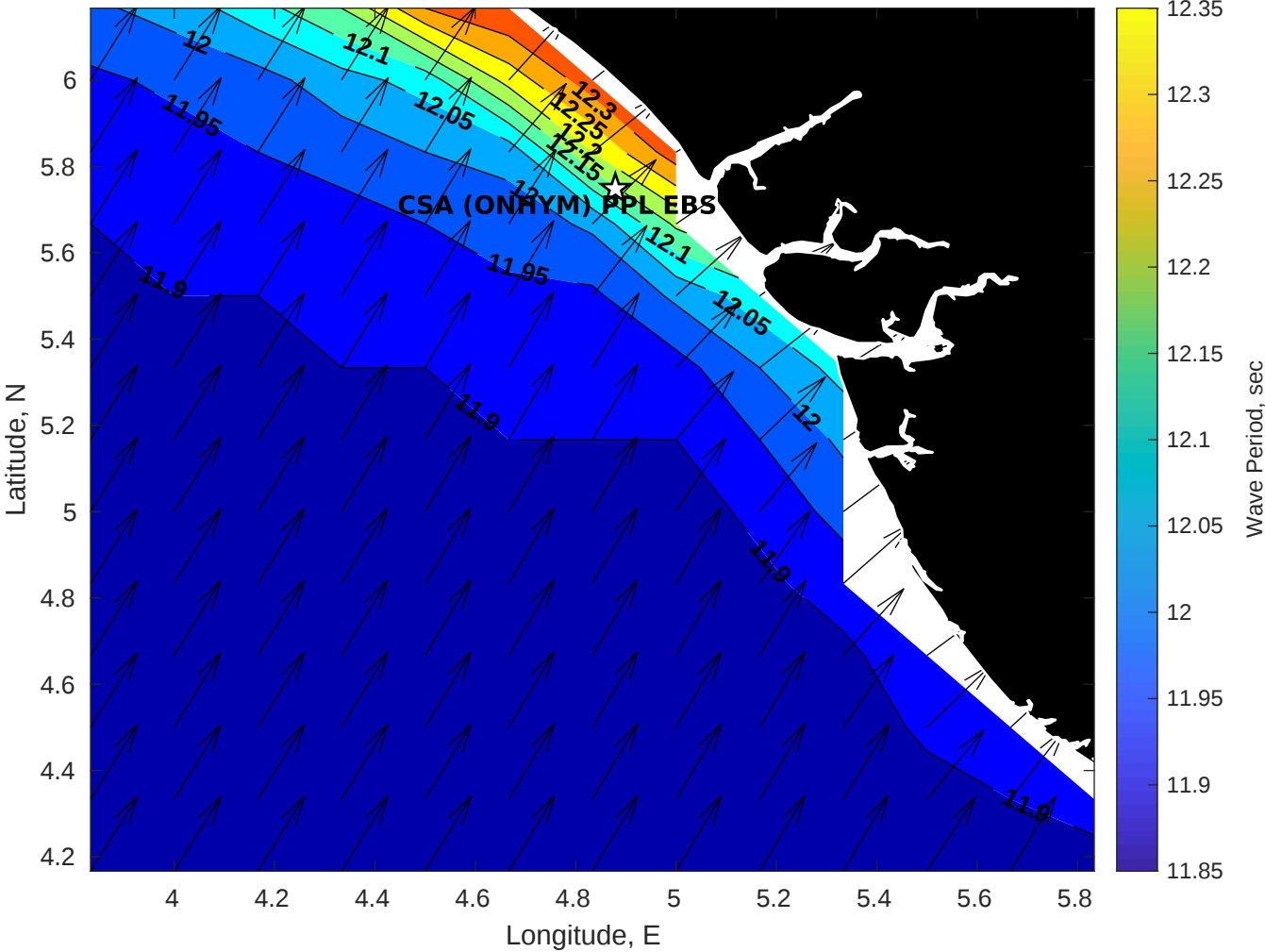
GFS Wave Period (sec) for CSA (ONHYM) PPL EBS - Nigeria at 16-Jan-2026 09:00:00
