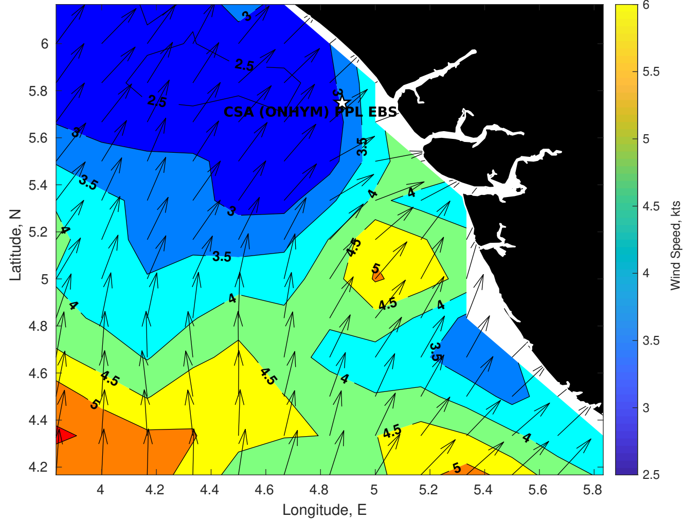
GFS Winds (kts) for CSA (ONHYM) PPL EBS - Nigeria at 16-Jan-2026 09:00:00
