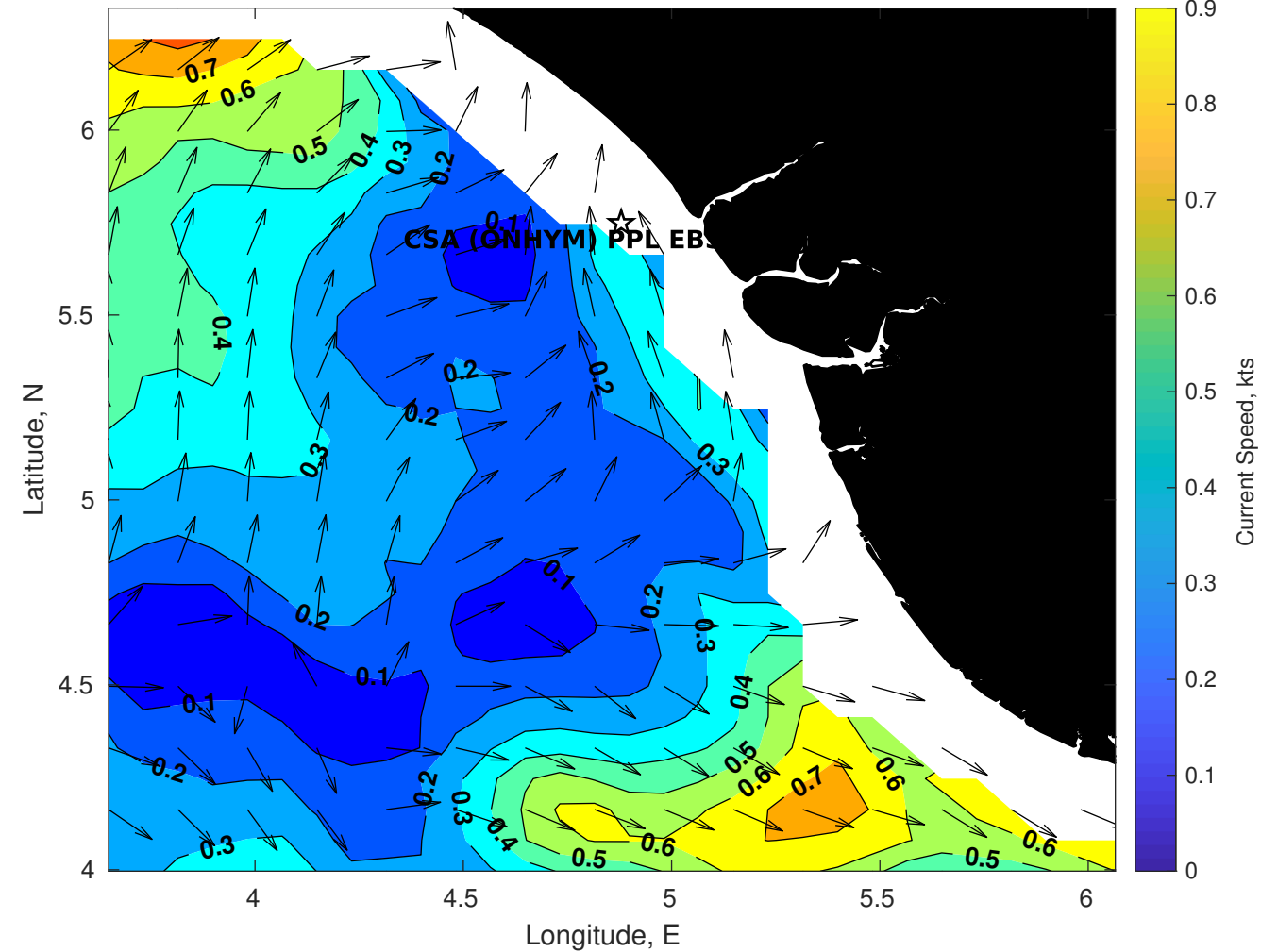
Surface Currents for CSA (ONHYM) PPL EBS - Nigeria at 15-Jan-2026 00:00:00
