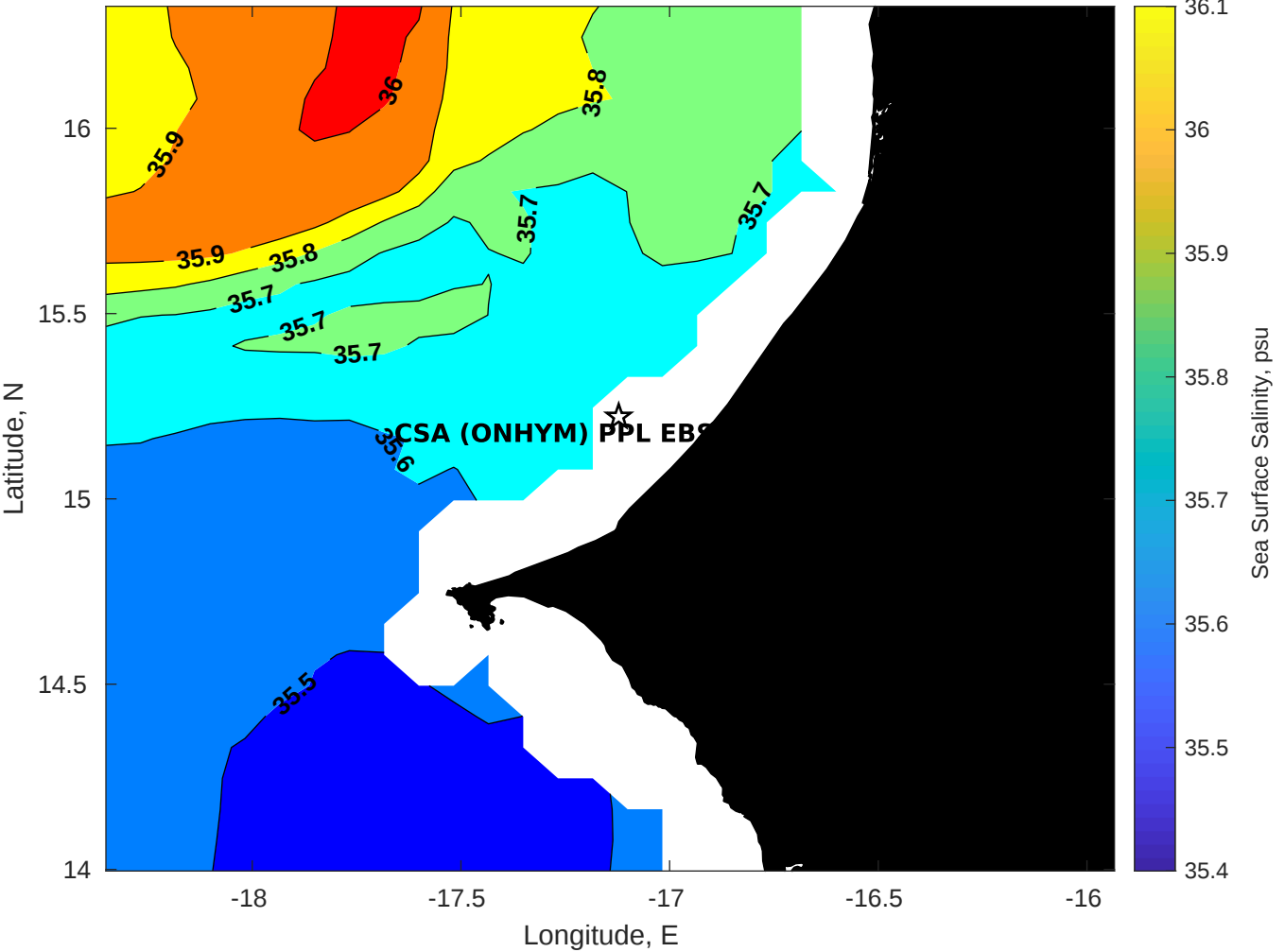
Surface Salinity for CSA (ONHYM) PPL EBS - Senegal at 15-Jan-2026 00:00:00
