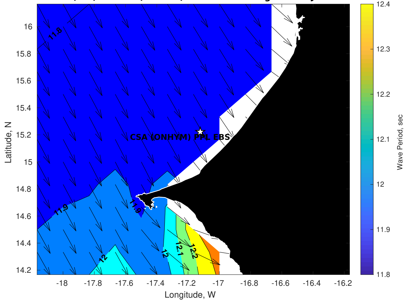
GFS Wave Period (sec) for CSA (ONHYM) PPL EBS - Senegal at 16-Jan-2026 09:00:00
