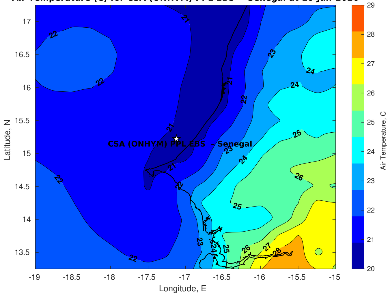
Air Temperature (C) for CSA (ONHYM) PPL EBS - Senegal at 16-Jan-2026
