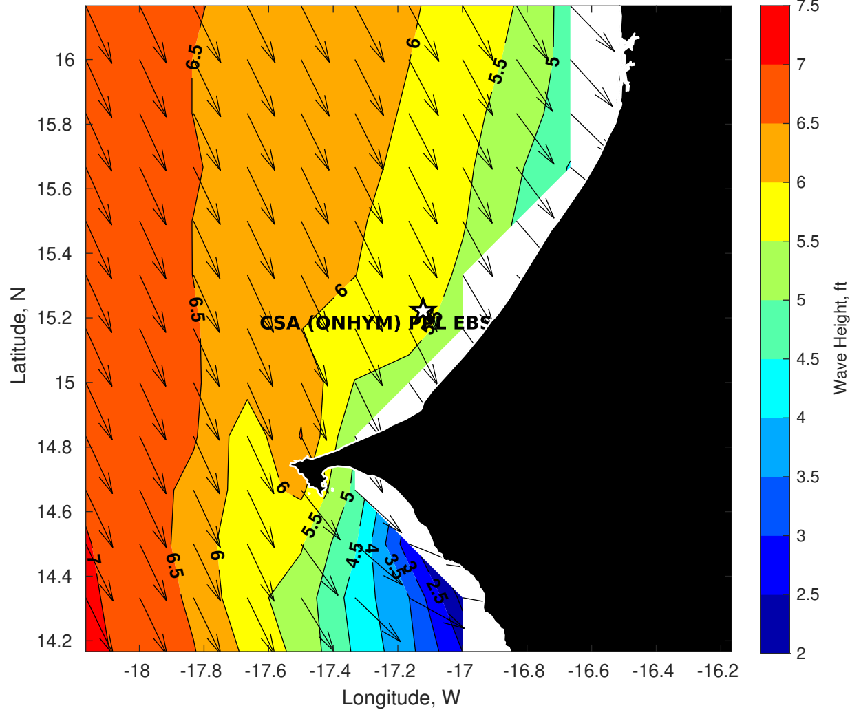
GFS Wave Height (ft) for CSA (ONHYM) PPL EBS - Senegal at 16-Jan-2026 09:00:00
