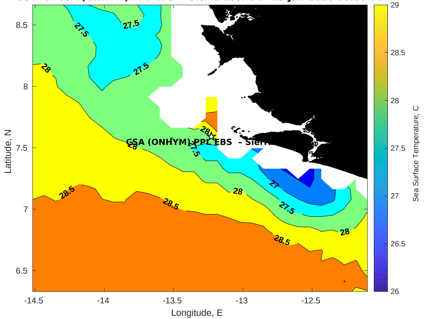
SST for CSA (ONHYM) PPL EBS - Sierra Leone at 15-Jan-2026 00:00:00
