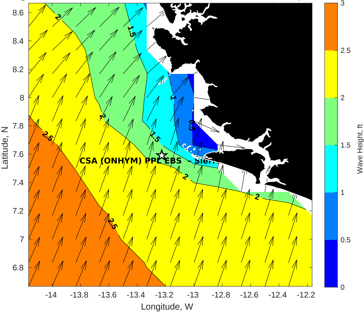
GFS Wave Height (ft) for CSA (ONHYM) PPL EBS - Sierra Leone at 16-Jan-2026 09:00:00
