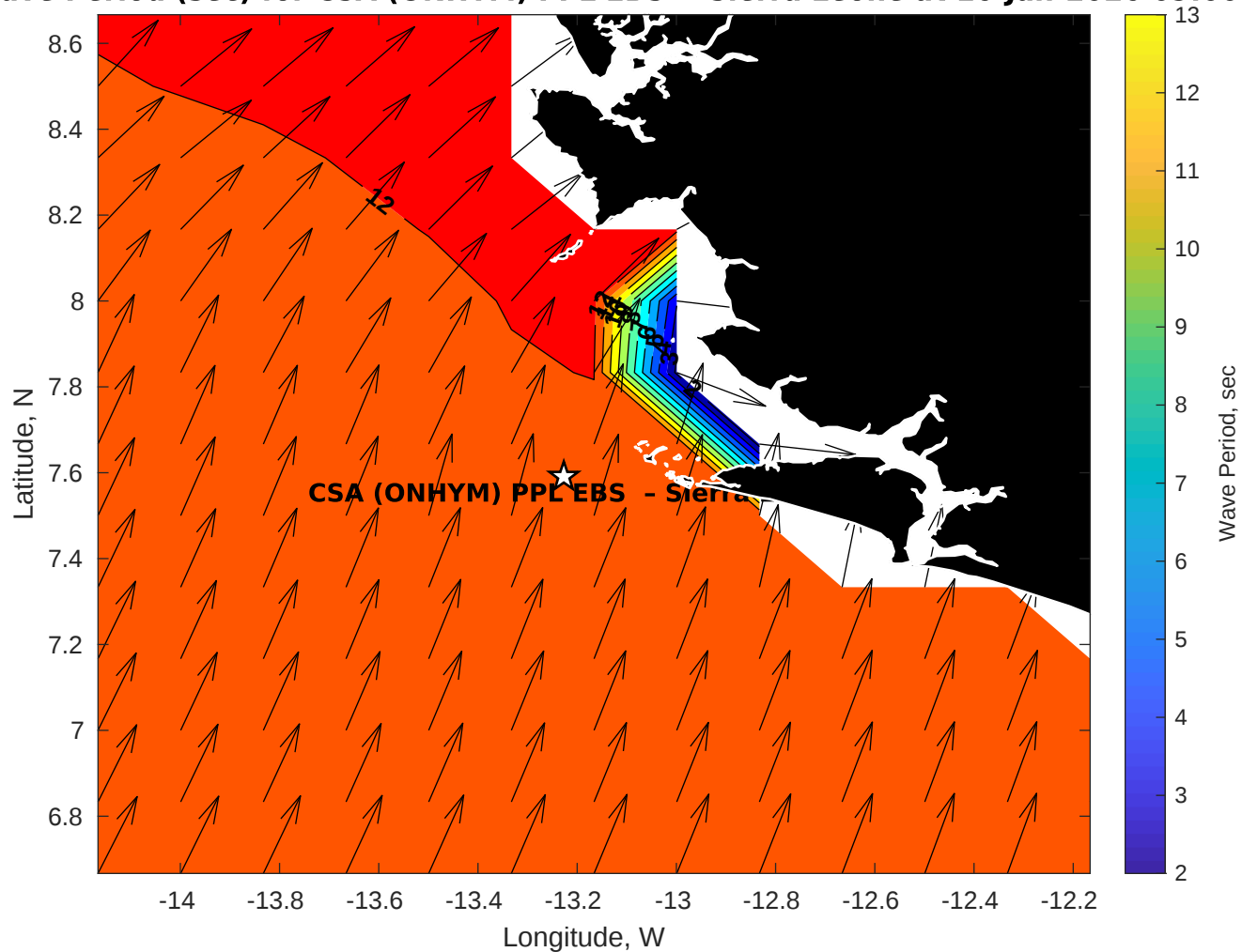
GFS Wave Period (sec) for CSA (ONHYM) PPL EBS - Sierra Leone at 16-Jan-2026 09:00:00
