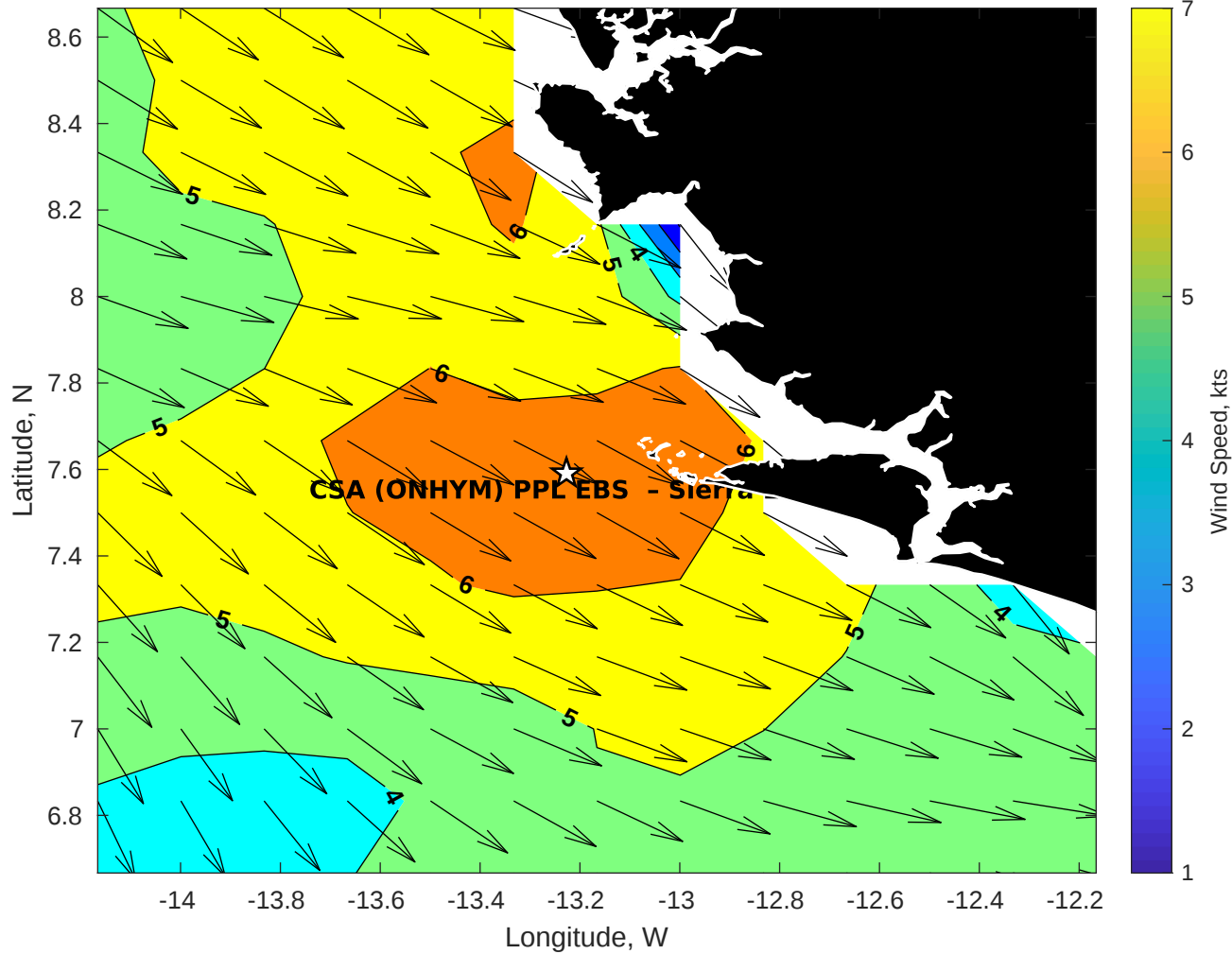
GFS Winds (kts) for CSA (ONHYM) PPL EBS - Sierra Leone at 16-Jan-2026 09:00:00
