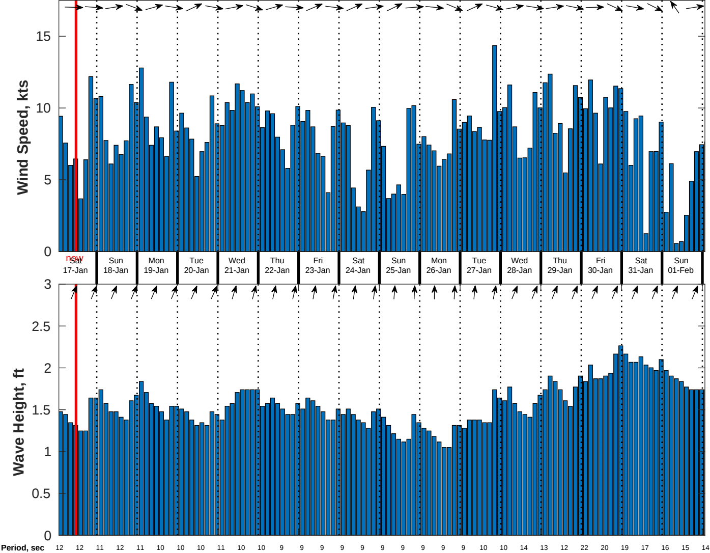
Wind & Wave Forecast for CSA (ONHYM) PPL EBS - Sierra Leone from 16-Jan-2026 01:00:00 to 01-Feb-2026 01:00:00
