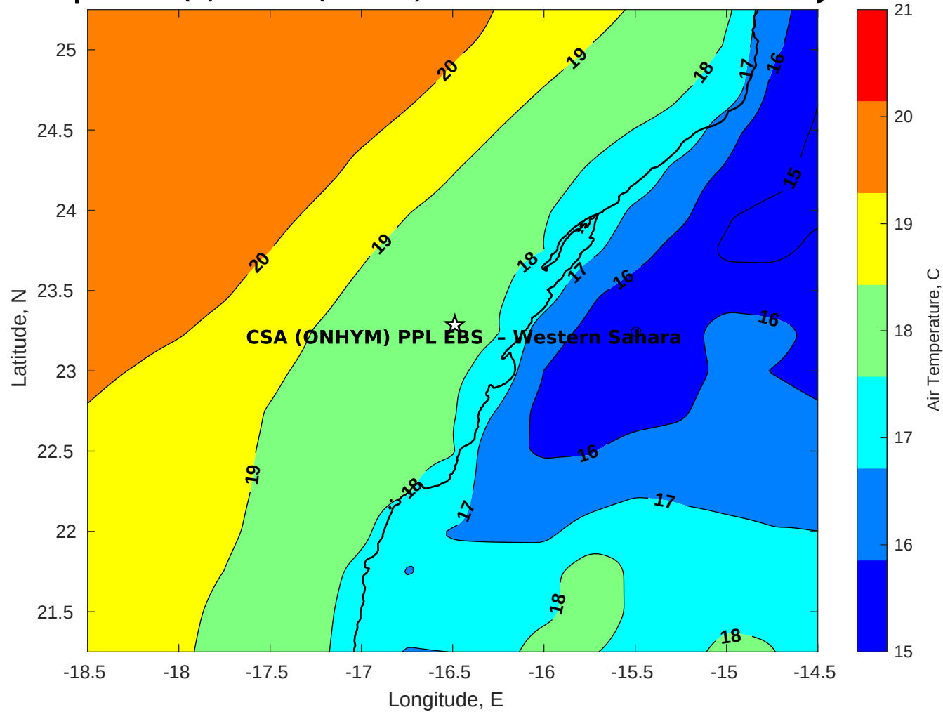
Air Temperature (C) for CSA (ONHYM) PPL EBS - Western Sahara at 16-Jan-2026
