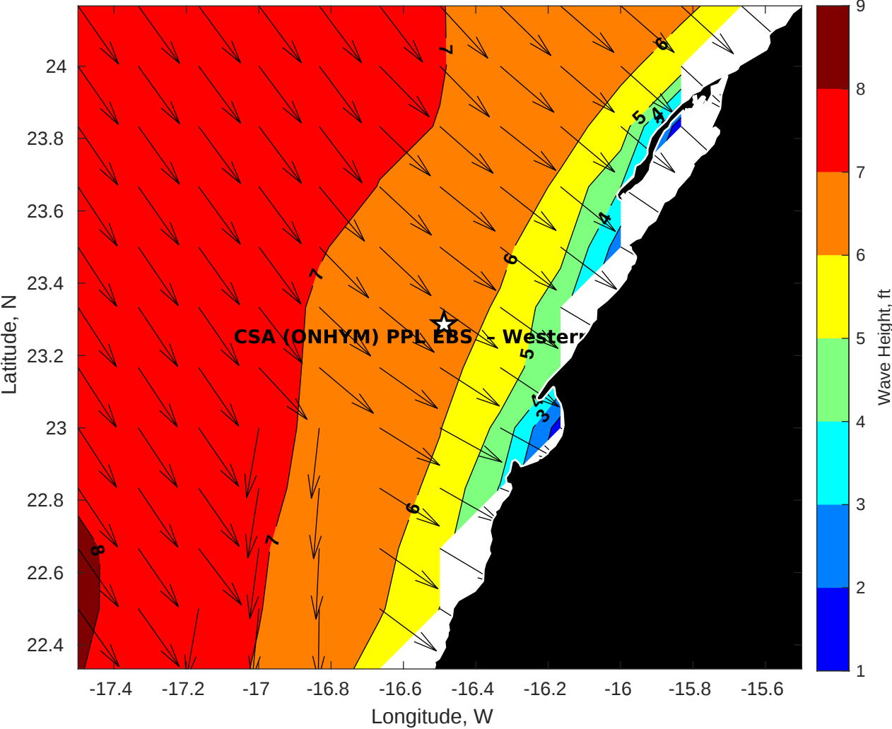
GFS Wave Height (ft) for CSA (ONHYM) PPL EBS - Western Sahara at 16-Jan-2026 09:00:00
