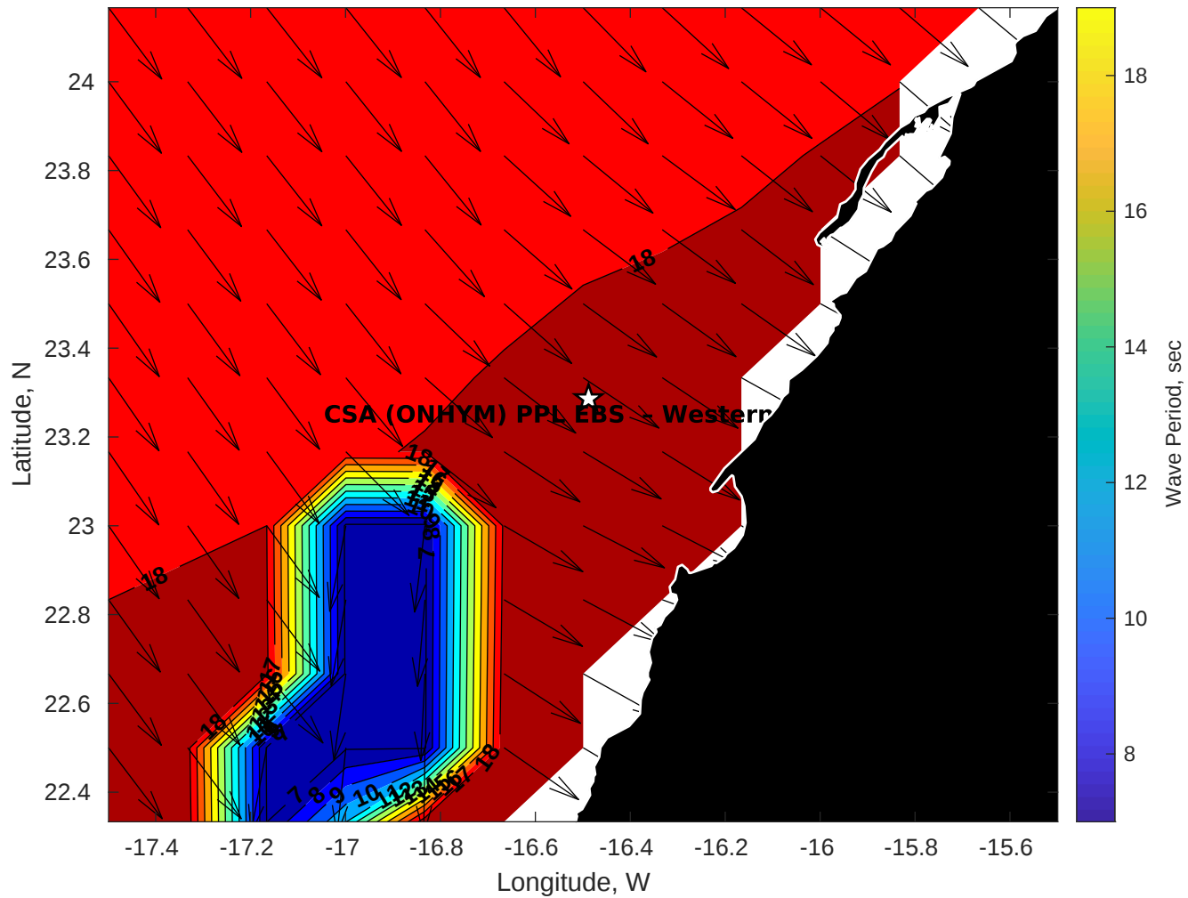
GFS Wave Period (sec) for CSA (ONHYM) PPL EBS - Western Sahara at 16-Jan-2026 09:00:00
