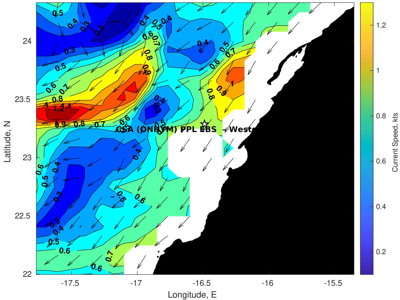
Surface Currents for CSA (ONHYM) PPL EBS - Western Sahara at 15-Jan-2026 00:00:00
