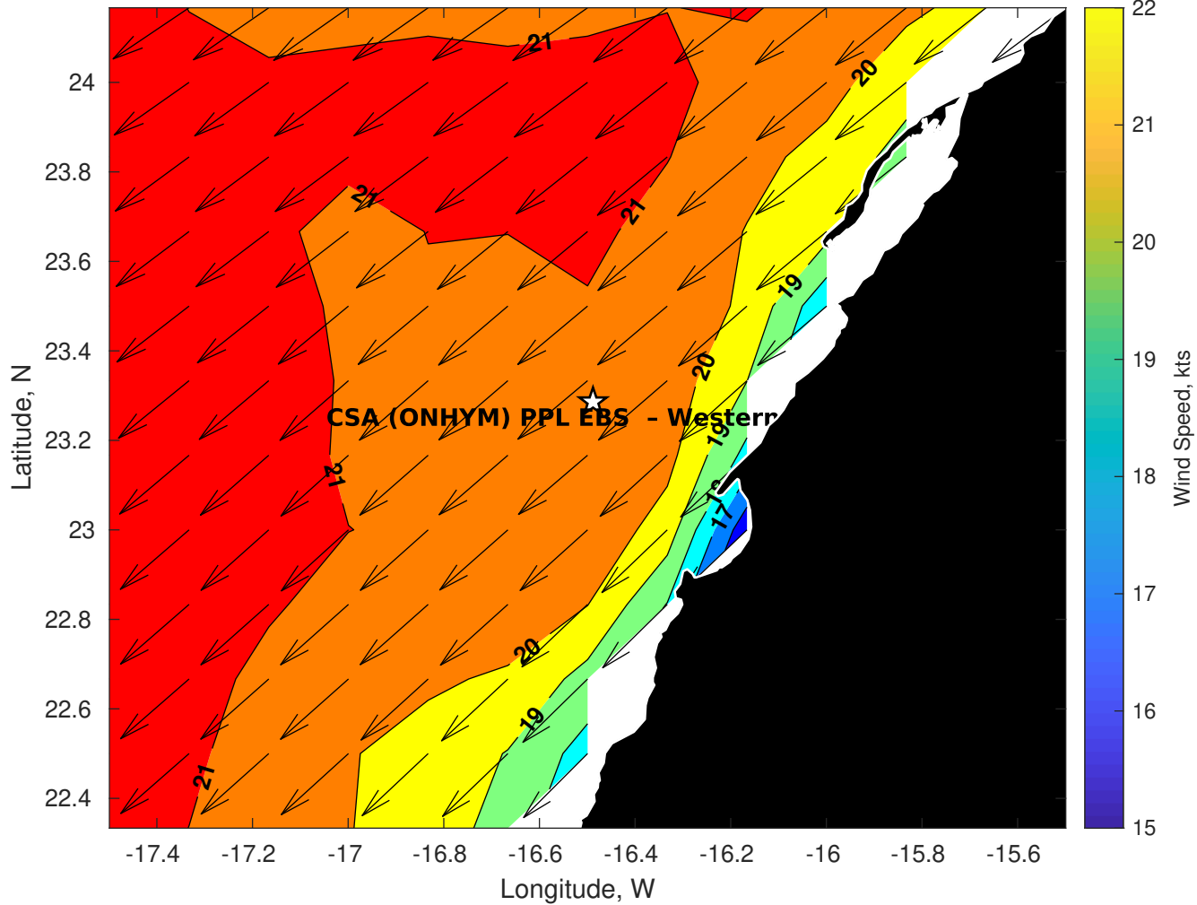
GFS Winds (kts) for CSA (ONHYM) PPL EBS - Western Sahara at 16-Jan-2026 09:00:00
