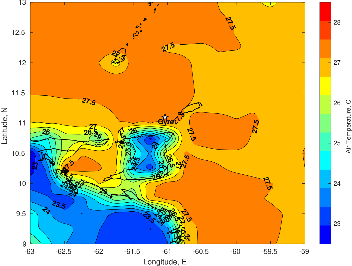
Air Temperature (C) for Gyre at 16-Jan-2026
