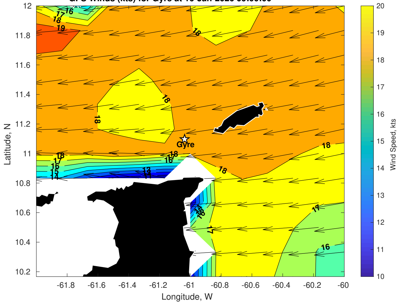
GFS Winds (kts) for Gyre at 16-Jan-2026 09:00:00
