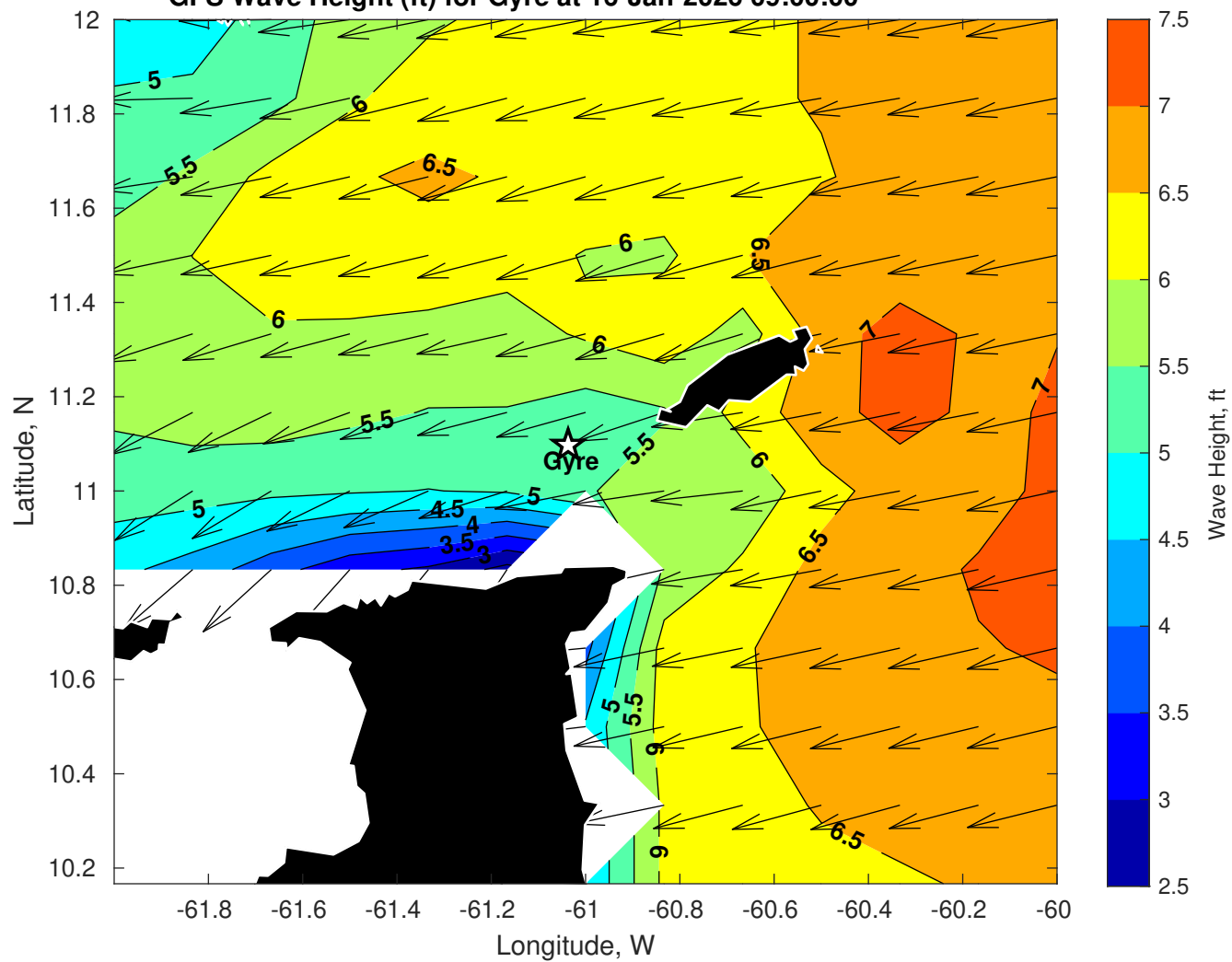
GFS Wave Height (ft) for Gyre at 16-Jan-2026 09:00:00
