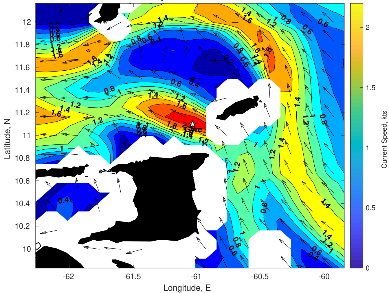
Surface Currents for Gyre at 15-Jan-2026 00:00:00
