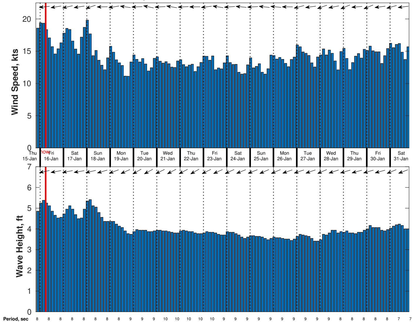
Wind & Wave Forecast for Gyre from 15-Jan-2026 20:00:00 to 31-Jan-2026 20:00:00
