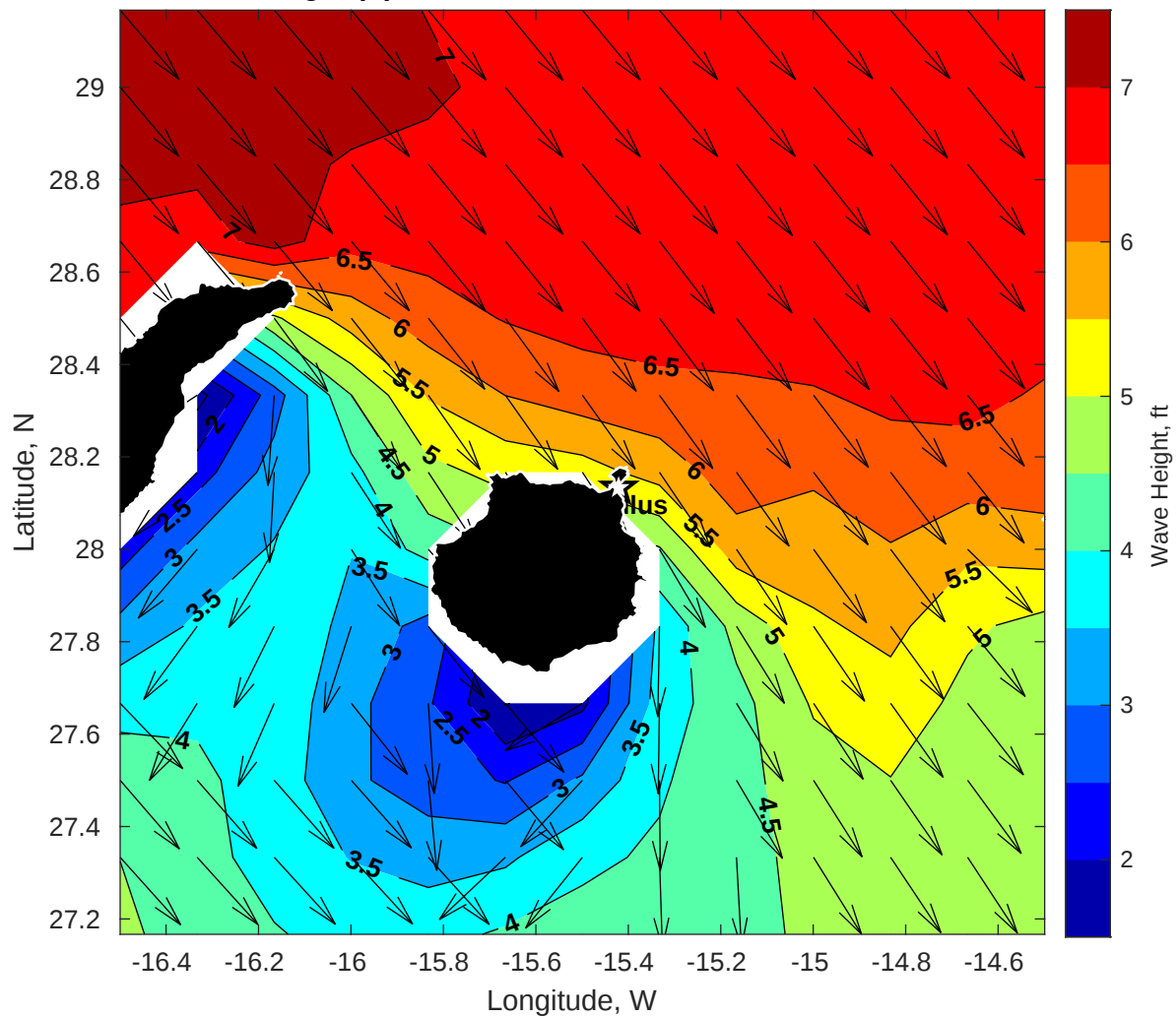
GFS Wave Height (ft) for Nautilus at 16-Jan-2026 09:00:00
