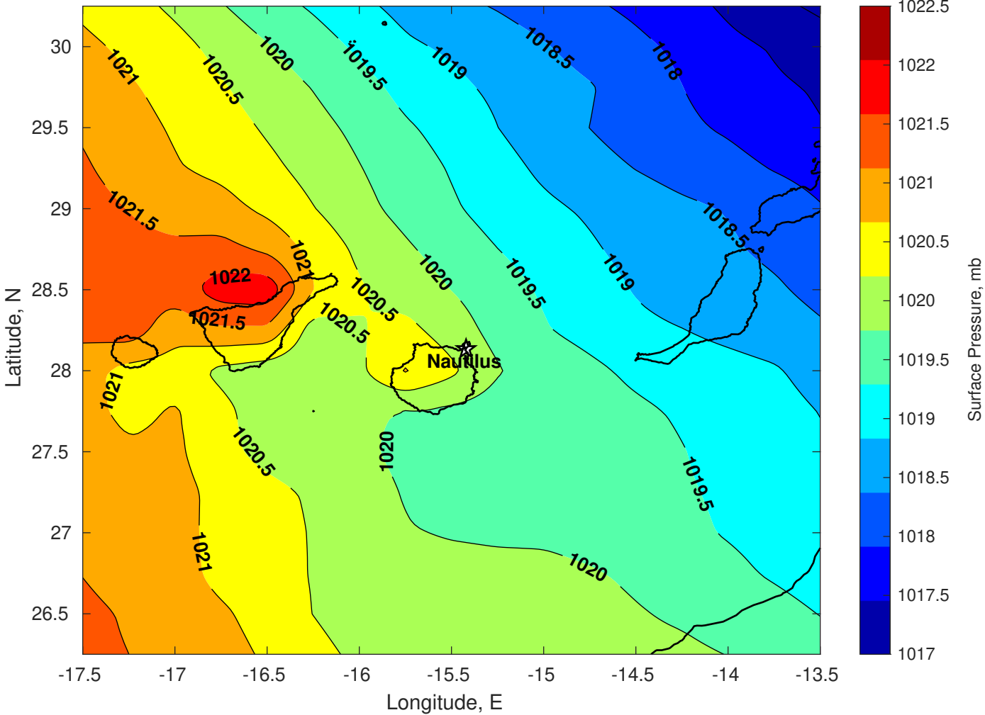
Surface Pressure (mb) for Nautilus at 18-Jan-2026 00:00:00
