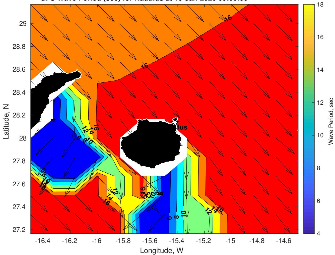
GFS Wave Period (sec) for Nautilus at 16-Jan-2026 09:00:00
