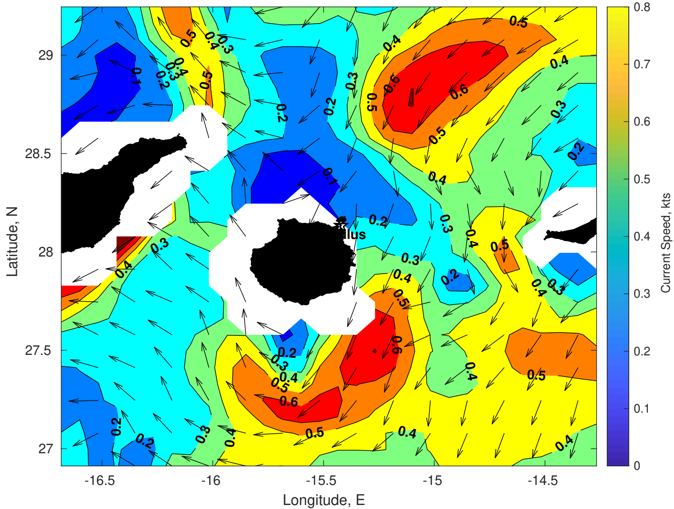
Surface Currents for Nautilus at 15-Jan-2026 00:00:00
