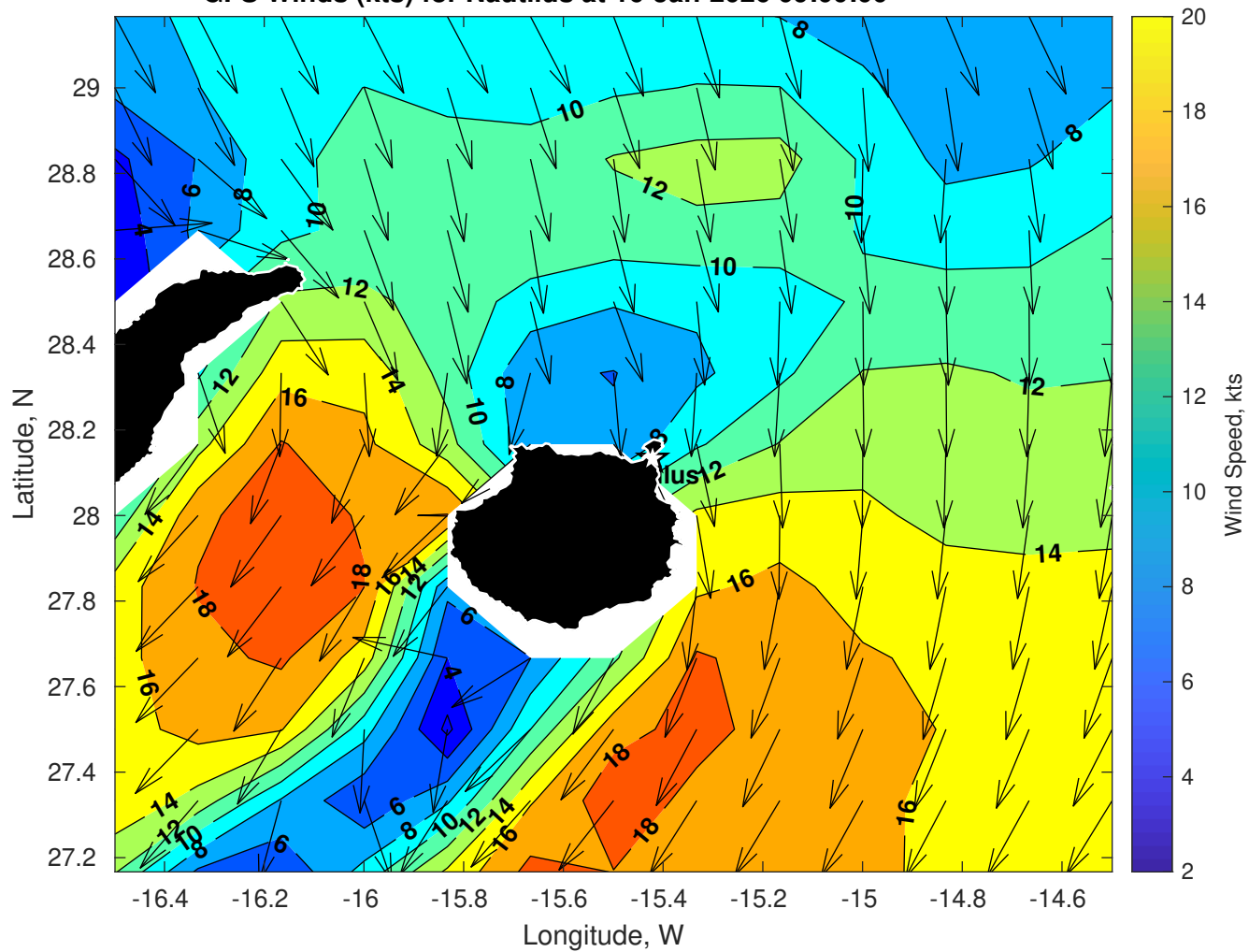
GFS Winds (kts) for Nautilus at 16-Jan-2026 09:00:00
