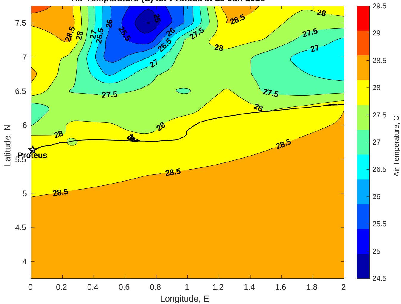
Air Temperature (C) for Proteus at 16-Jan-2026
