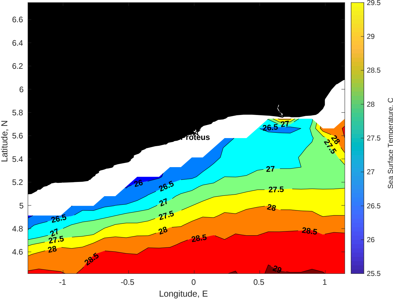
SST for Proteus at 15-Jan-2026 00:00:00
