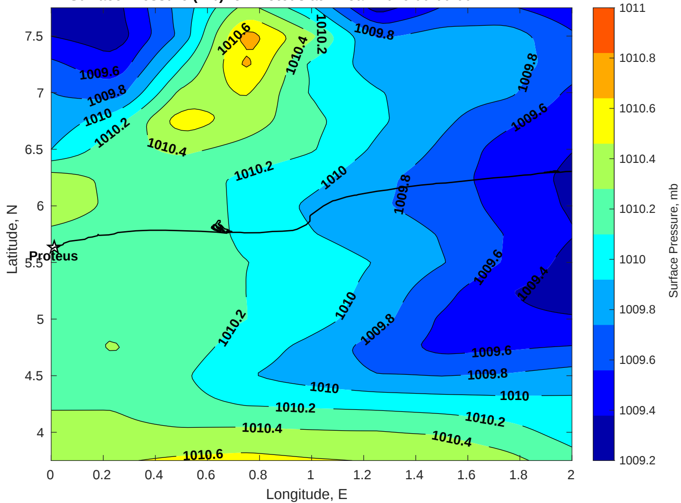
Surface Pressure (mb) for Proteus at 17-Jan-2026 00:00:00
