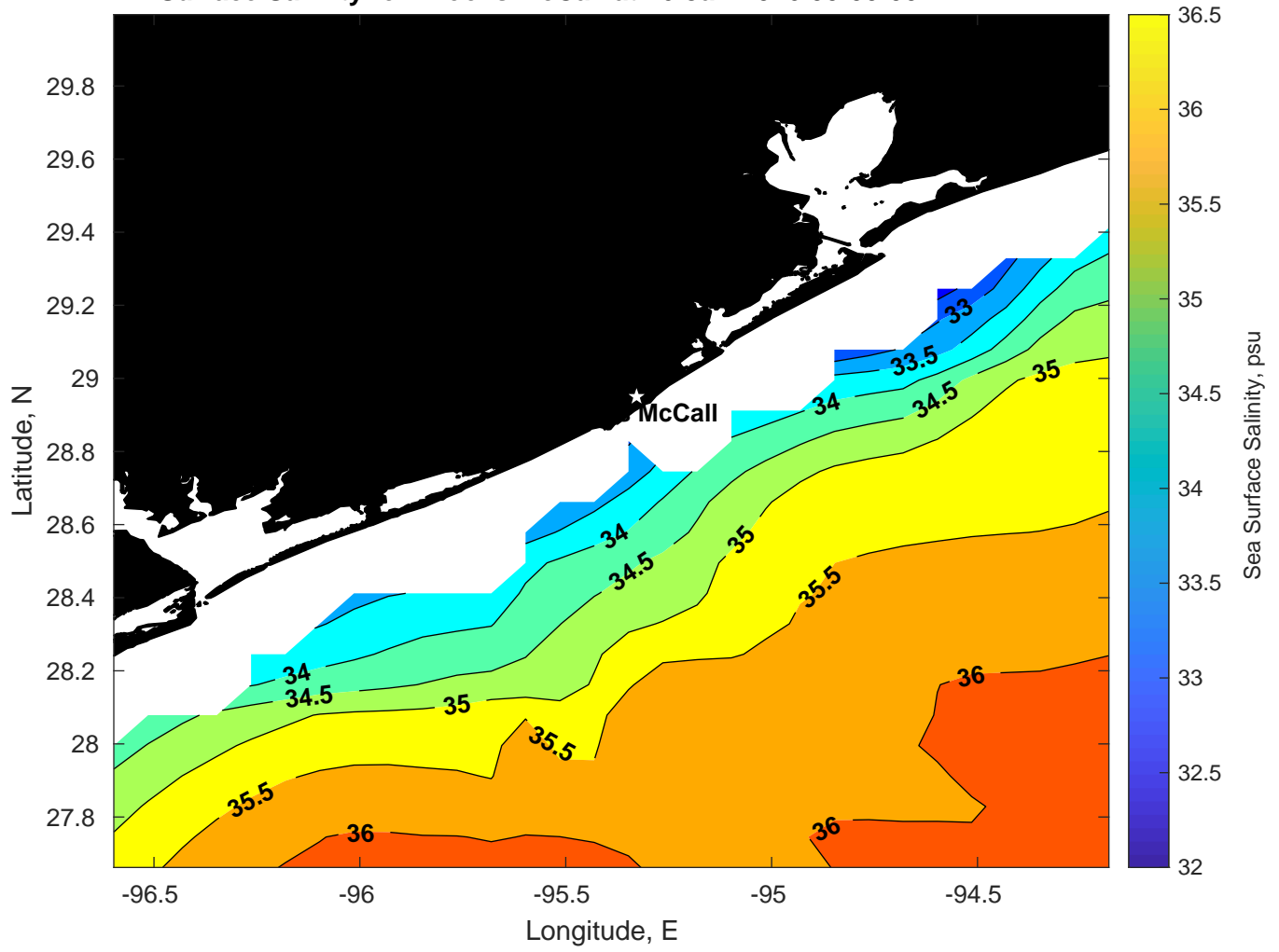
Surface Salinity for Brooks McCall at 16-Jan-2026 00:00:00
